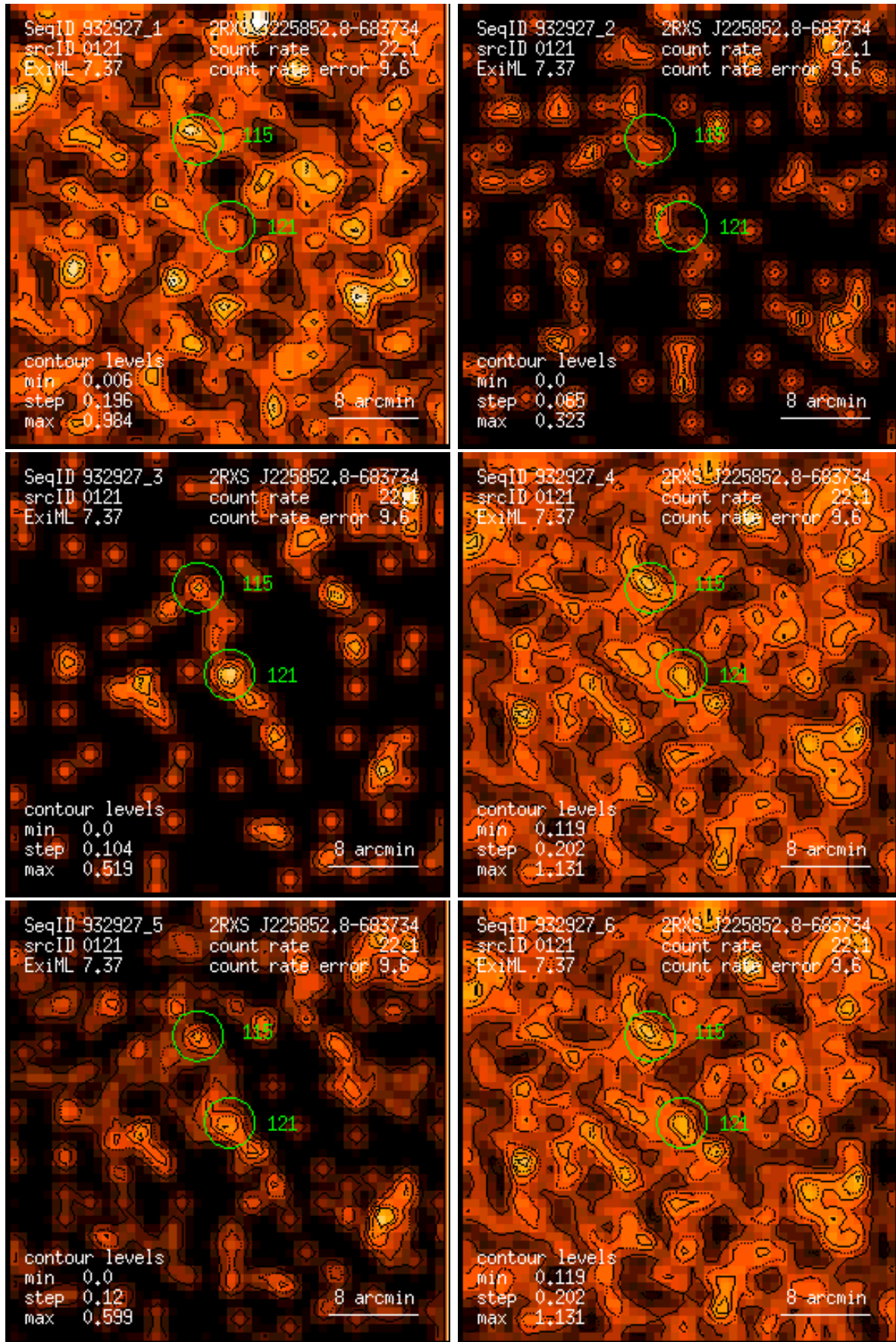
Figure 121: RASS 932927: detection 0121: band rate images, Gaussian filter: (1) PSPC channels 11 – 41, (2) 52 – 90, (3) 91 – 201, (4) 11 – 235, (5) 52 – 201, (6) 11 – 201. Broad band rates in counts/ks. Band rate contour levels in counts/ks/arcmin 2 .
