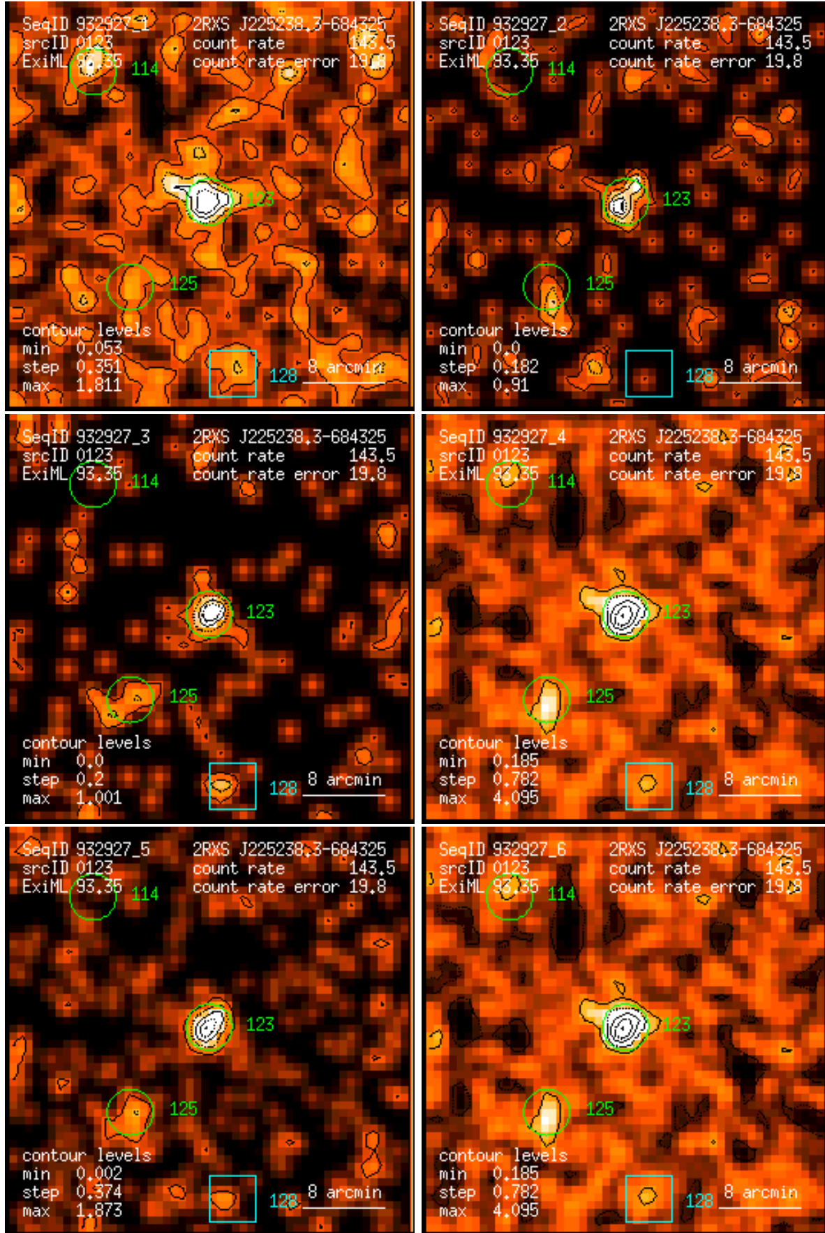
Figure 123: RASS 932927: detection 0123: band rate images, Gaussian filter: (1) PSPC channels 11 – 41, (2) 52 – 90, (3) 91 – 201, (4) 11 – 235, (5) 52 – 201, (6) 11 – 201. Broad band rates in counts/ks. Band rate contour levels in counts/ks/arcmin 2 .
