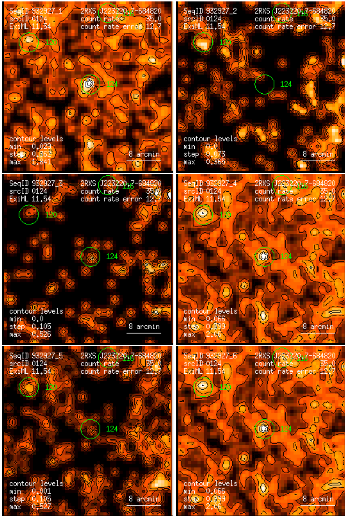
Figure 124: RASS 932927: detection 0124: band rate images, Gaussian filter: (1) PSPC channels 11 – 41, (2) 52 – 90, (3) 91 – 201, (4) 11 – 235, (5) 52 – 201, (6) 11 – 201. Broad band rates in counts/ks. Band rate contour levels in counts/ks/arcmin 2 .
