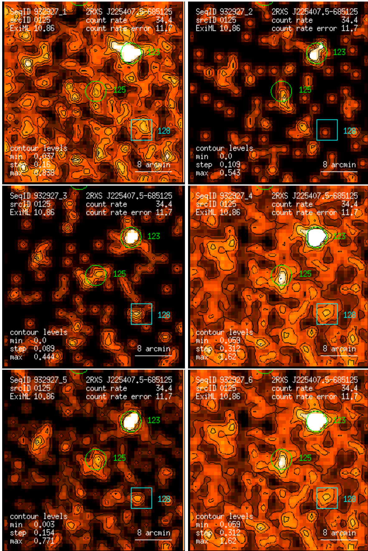
Figure 125: RASS 932927: detection 0125: band rate images, Gaussian filter: (1) PSPC channels 11 – 41, (2) 52 – 90, (3) 91 – 201, (4) 11 – 235, (5) 52 – 201, (6) 11 – 201. Broad band rates in counts/ks. Band rate contour levels in counts/ks/arcmin 2 .
