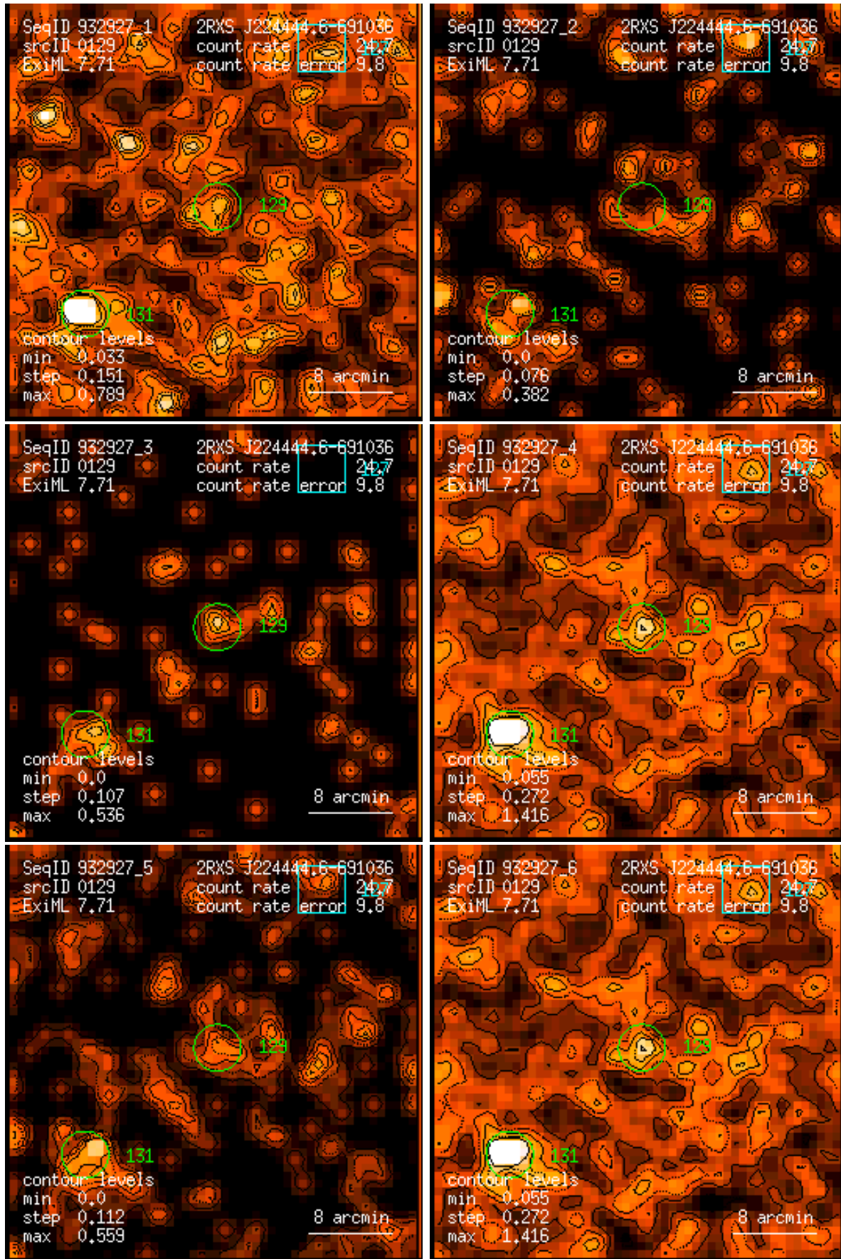
Figure 129: RASS 932927: detection 0129: band rate images, Gaussian filter: (1) PSPC channels 11 – 41, (2) 52 – 90, (3) 91 – 201, (4) 11 – 235, (5) 52 – 201, (6) 11 – 201. Broad band rates in counts/ks. Band rate contour levels in counts/ks/arcmin 2 .
