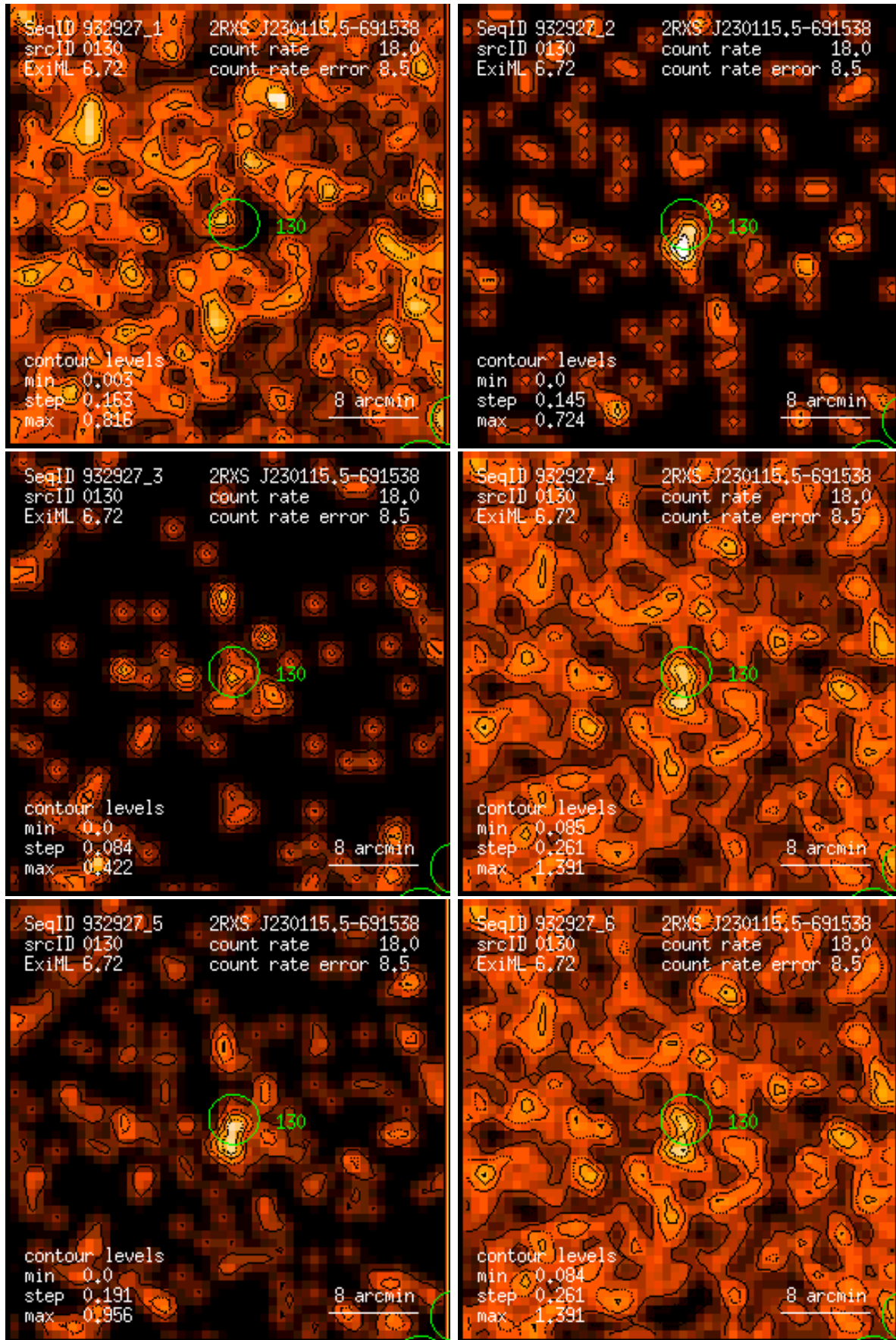
Figure 130: RASS 932927: detection 0130: band rate images, Gaussian filter: (1) PSPC channels 11 – 41, (2) 52 – 90, (3) 91 – 201, (4) 11 – 235, (5) 52 – 201, (6) 11 – 201. Broad band rates in counts/ks. Band rate contour levels in counts/ks/arcmin 2 .
