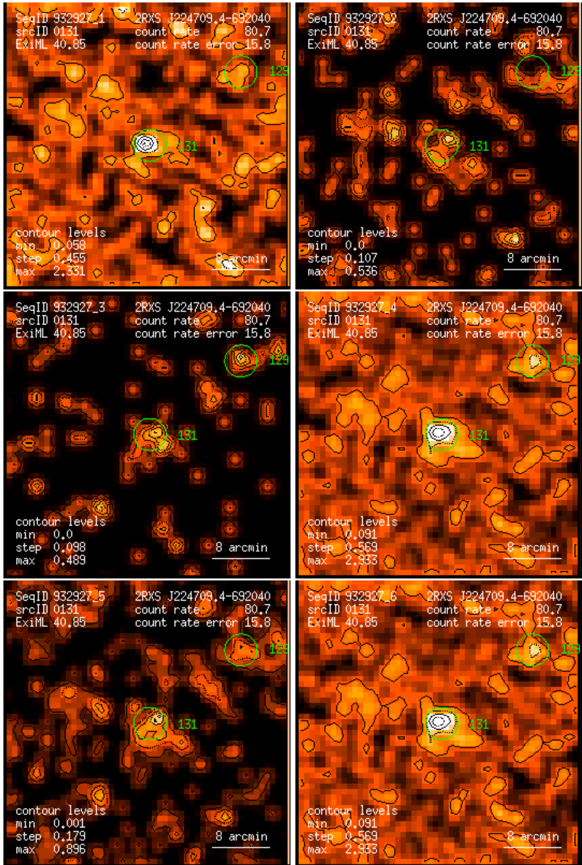
Figure 131: RASS 932927: detection 0131: band rate images, Gaussian filter: (1) PSPC channels 11 – 41, (2) 52 – 90, (3) 91 – 201, (4) 11 – 235, (5) 52 – 201, (6) 11 – 201. Broad band rates in counts/ks. Band rate contour levels in counts/ks/arcmin 2 .
