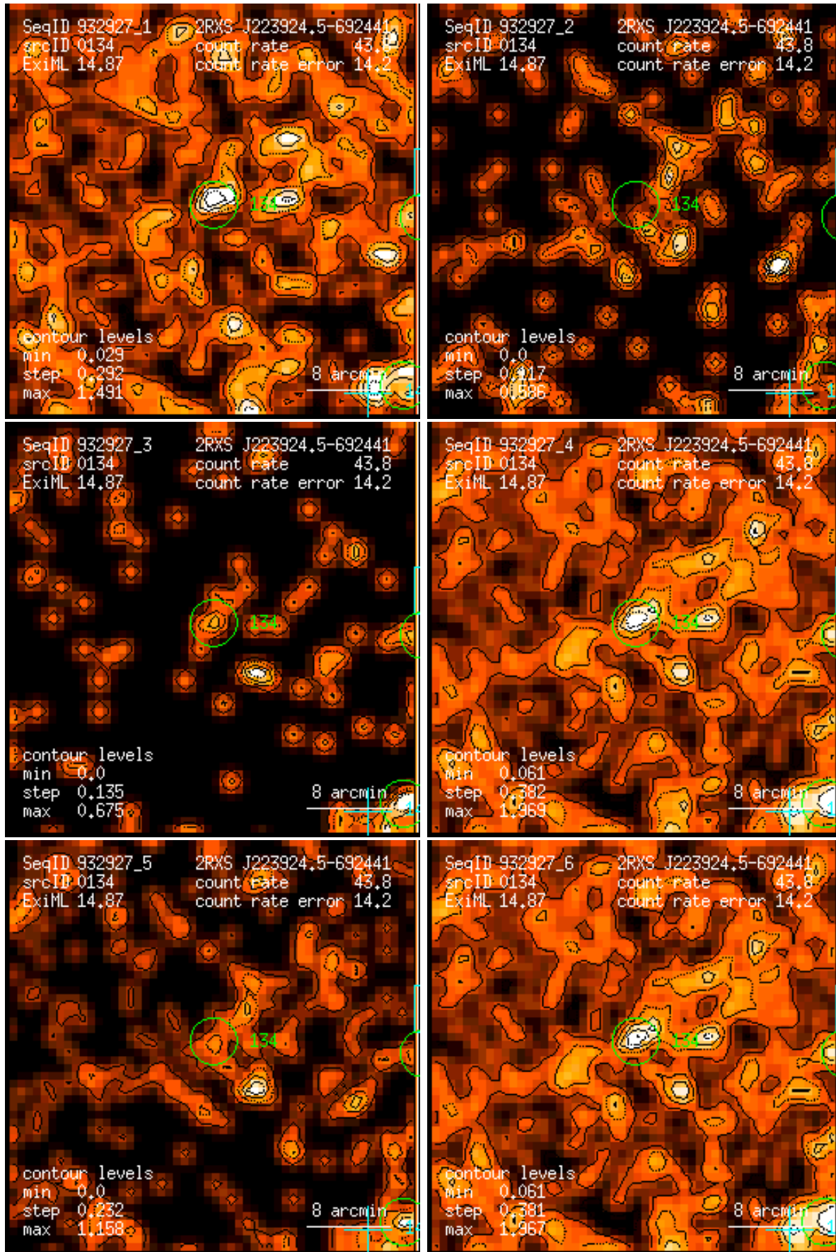
Figure 134: RASS 932927: detection 0134: band rate images, Gaussian filter: (1) PSPC channels 11 – 41, (2) 52 – 90, (3) 91 – 201, (4) 11 – 235, (5) 52 – 201, (6) 11 – 201. Broad band rates in counts/ks. Band rate contour levels in counts/ks/arcmin 2 .
