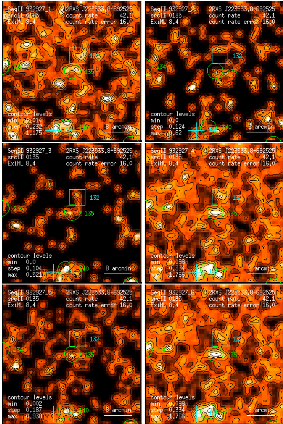
Figure 135: RASS 932927: detection 0135: band rate images, Gaussian filter: (1) PSPC channels 11 – 41, (2) 52 – 90, (3) 91 – 201, (4) 11 – 235, (5) 52 – 201, (6) 11 – 201. Broad band rates in counts/ks. Band rate contour levels in counts/ks/arcmin 2 .
