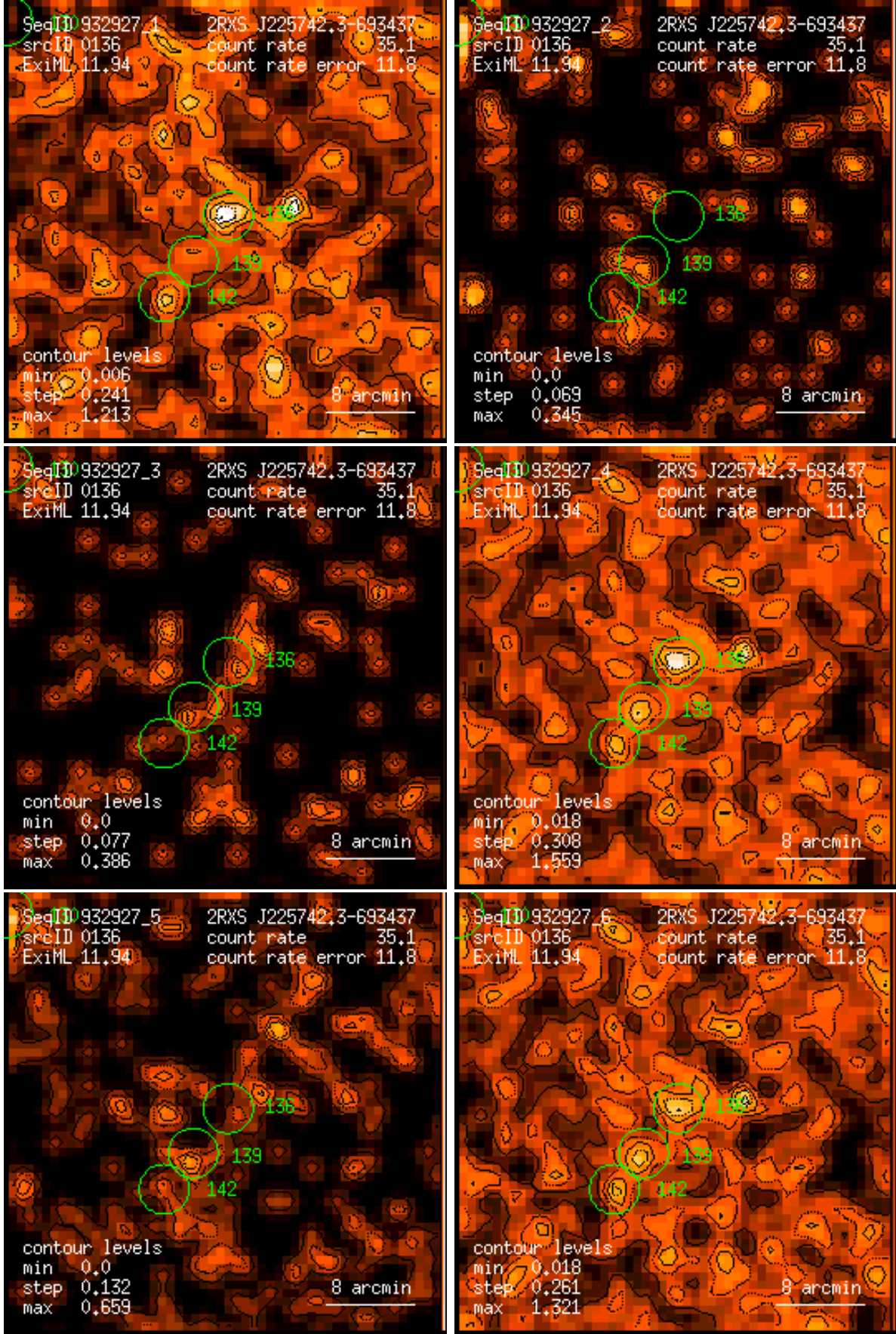
Figure 136: RASS 932927: detection 0136: band rate images, Gaussian filter: (1) PSPC channels 11 – 41, (2) 52 – 90, (3) 91 – 201, (4) 11 – 235, (5) 52 – 201, (6) 11 – 201. Broad band rates in counts/ks. Band rate contour levels in counts/ks/arcmin 2 .
