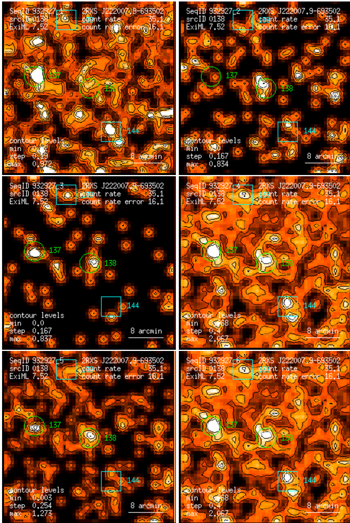
Figure 138: RASS 932927: detection 0138: band rate images, Gaussian filter: (1) PSPC channels 11 – 41, (2) 52 – 90, (3) 91 – 201, (4) 11 – 235, (5) 52 – 201, (6) 11 – 201. Broad band rates in counts/ks. Band rate contour levels in counts/ks/arcmin 2 .
