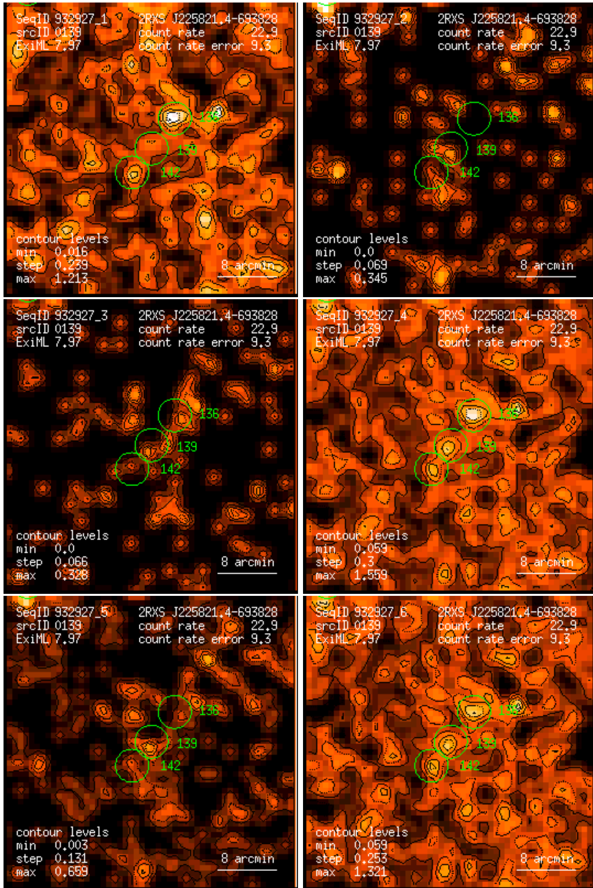
Figure 139: RASS 932927: detection 0139: band rate images, Gaussian filter: (1) PSPC channels 11 – 41, (2) 52 – 90, (3) 91 – 201, (4) 11 – 235, (5) 52 – 201, (6) 11 – 201. Broad band rates in counts/ks. Band rate contour levels in counts/ks/arcmin 2 .
