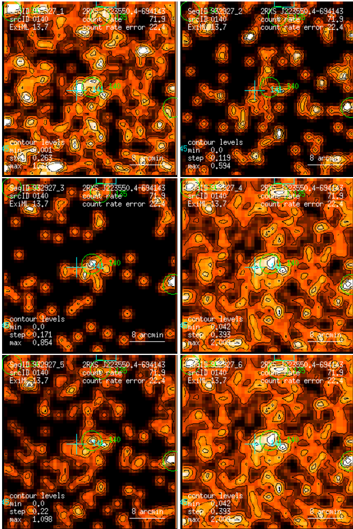
Figure 140: RASS 932927: detection 0140: band rate images, Gaussian filter: (1) PSPC channels 11 – 41, (2) 52 – 90, (3) 91 – 201, (4) 11 – 235, (5) 52 – 201, (6) 11 – 201. Broad band rates in counts/ks. Band rate contour levels in counts/ks/arcmin 2 .
