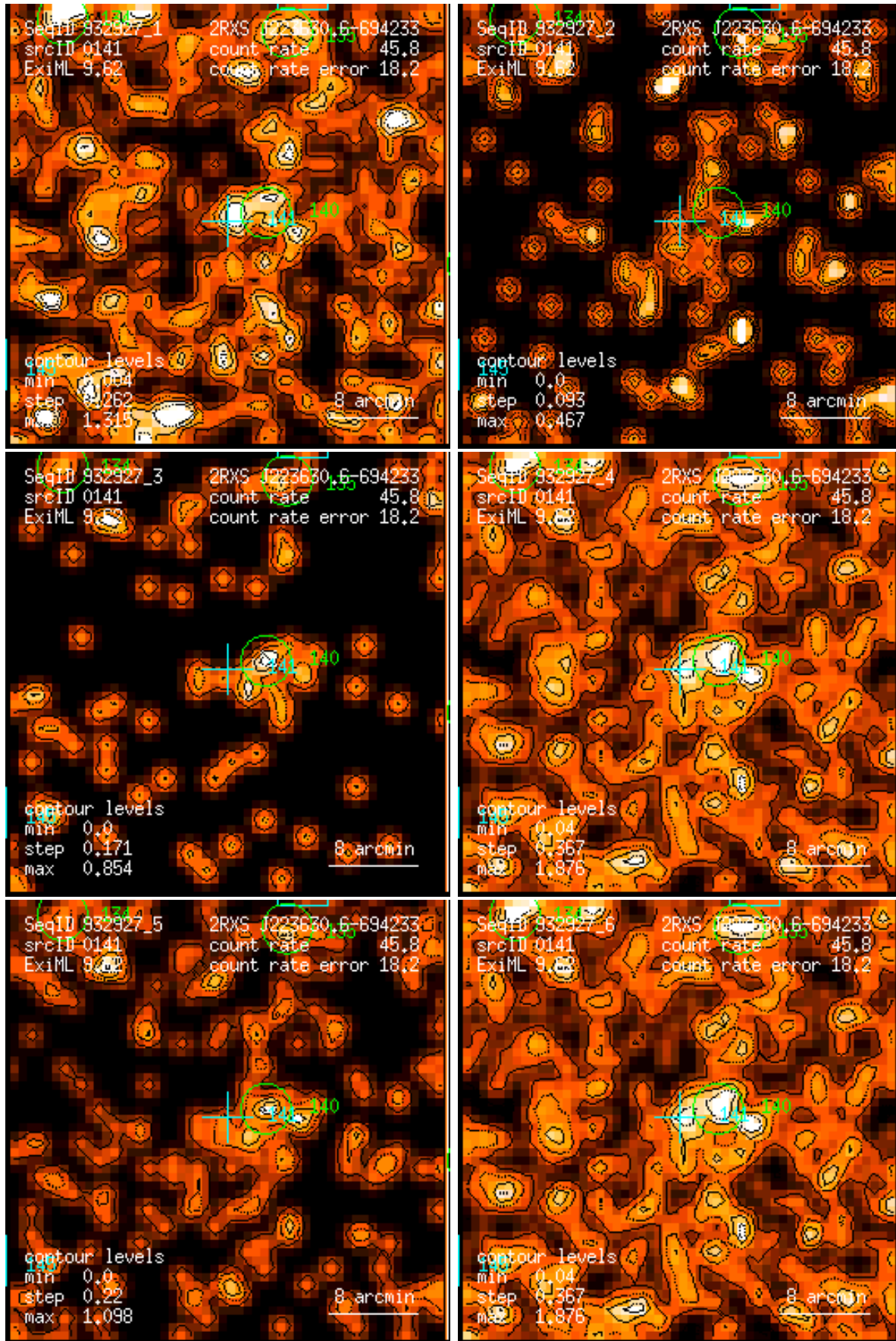
Figure 141: RASS 932927: detection 0141: band rate images, Gaussian filter: (1) PSPC channels 11 – 41, (2) 52 – 90, (3) 91 – 201, (4) 11 – 235, (5) 52 – 201, (6) 11 – 201. Broad band rates in counts/ks. Band rate contour levels in counts/ks/arcmin 2 .
