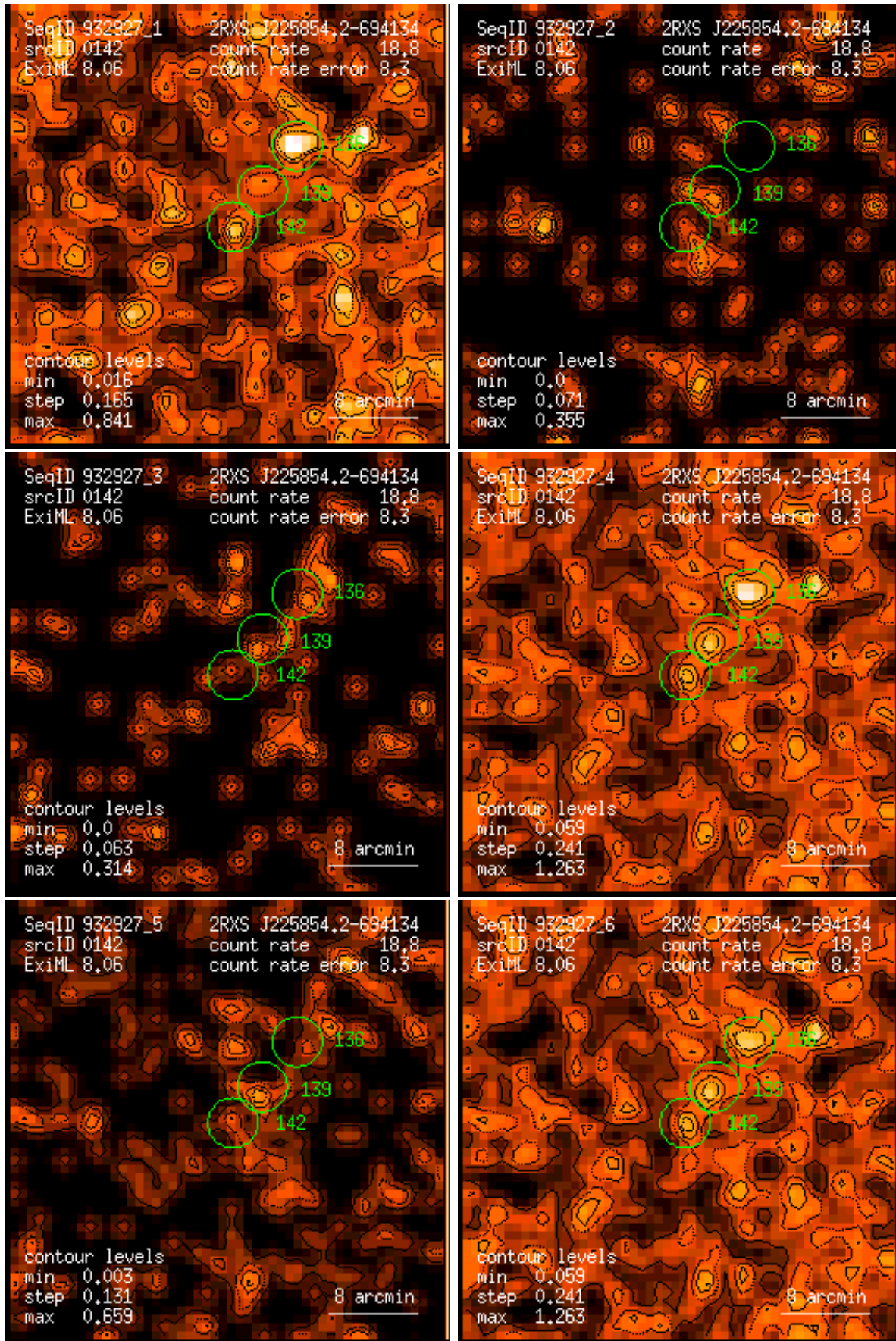
Figure 142: RASS 932927: detection 0142: band rate images, Gaussian filter: (1) PSPC channels 11 – 41, (2) 52 – 90, (3) 91 – 201, (4) 11 – 235, (5) 52 – 201, (6) 11 – 201. Broad band rates in counts/ks. Band rate contour levels in counts/ks/arcmin 2 .
