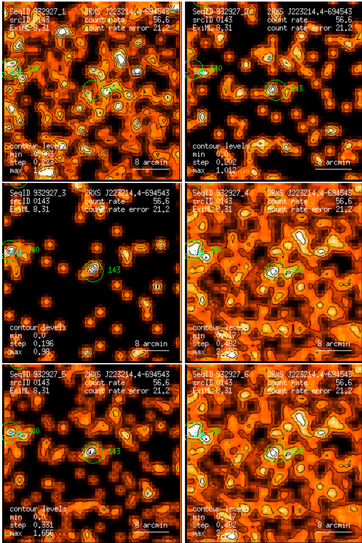
Figure 143: RASS 932927: detection 0143: band rate images, Gaussian filter: (1) PSPC channels 11 – 41, (2) 52 – 90, (3) 91 – 201, (4) 11 – 235, (5) 52 – 201, (6) 11 – 201. Broad band rates in counts/ks. Band rate contour levels in counts/ks/arcmin 2 .
