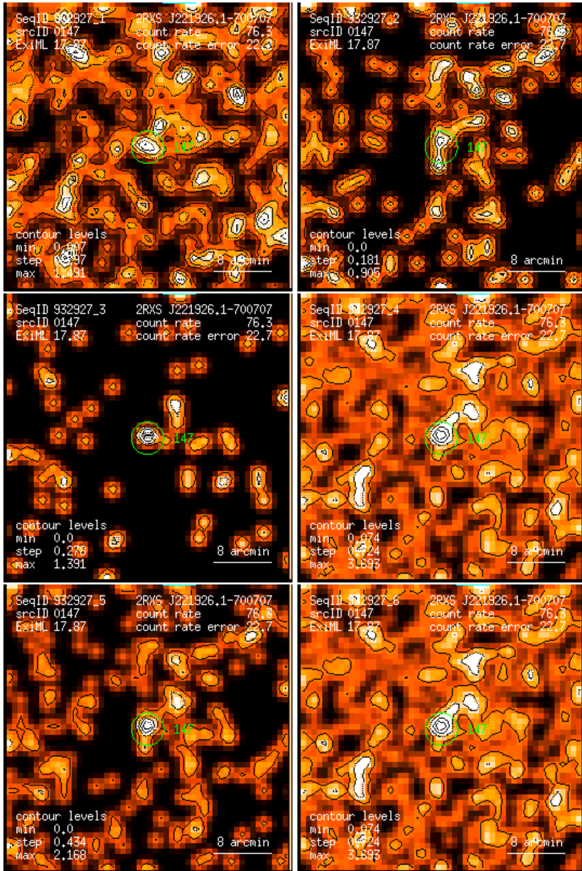
Figure 147: RASS 932927: detection 0147: band rate images, Gaussian filter: (1) PSPC channels 11 – 41, (2) 52 – 90, (3) 91 – 201, (4) 11 – 235, (5) 52 – 201, (6) 11 – 201. Broad band rates in counts/ks. Band rate contour levels in counts/ks/arcmin 2 .
