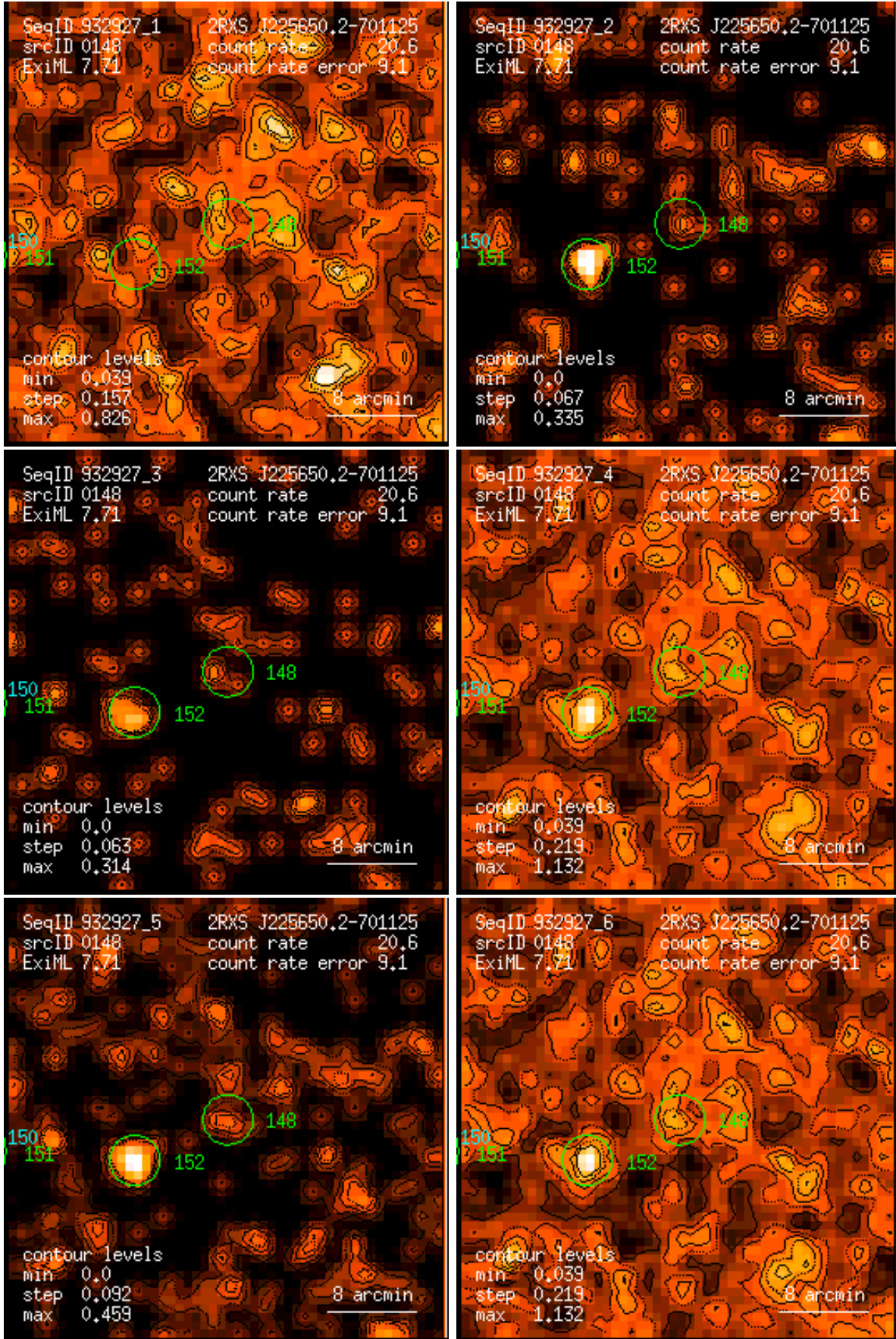
Figure 148: RASS 932927: detection 0148: band rate images, Gaussian filter: (1) PSPC channels 11 – 41, (2) 52 – 90, (3) 91 – 201, (4) 11 – 235, (5) 52 – 201, (6) 11 – 201. Broad band rates in counts/ks. Band rate contour levels in counts/ks/arcmin 2 .
