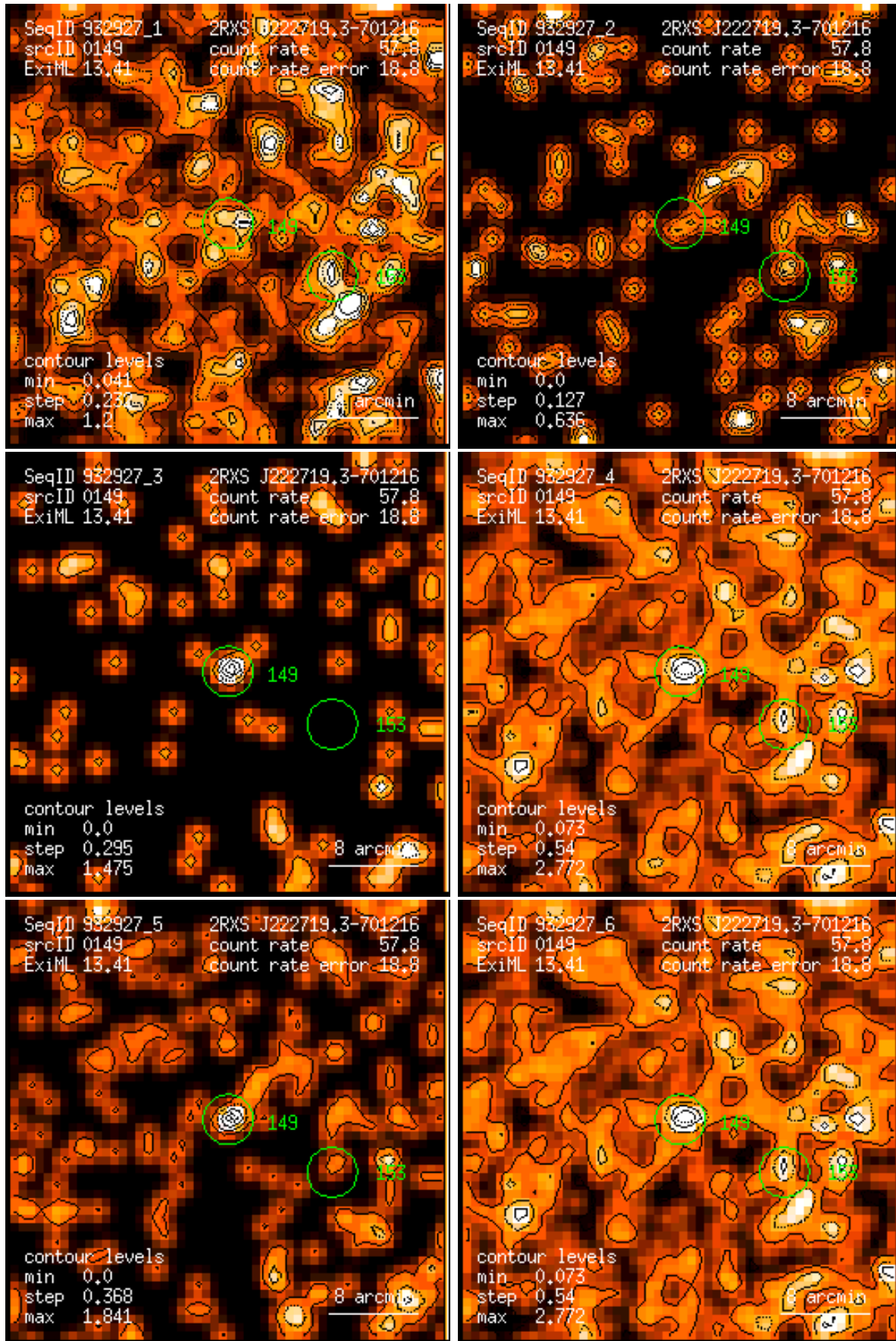
Figure 149: RASS 932927: detection 0149: band rate images, Gaussian filter: (1) PSPC channels 11 – 41, (2) 52 – 90, (3) 91 – 201, (4) 11 – 235, (5) 52 – 201, (6) 11 – 201. Broad band rates in counts/ks. Band rate contour levels in counts/ks/arcmin 2 .
