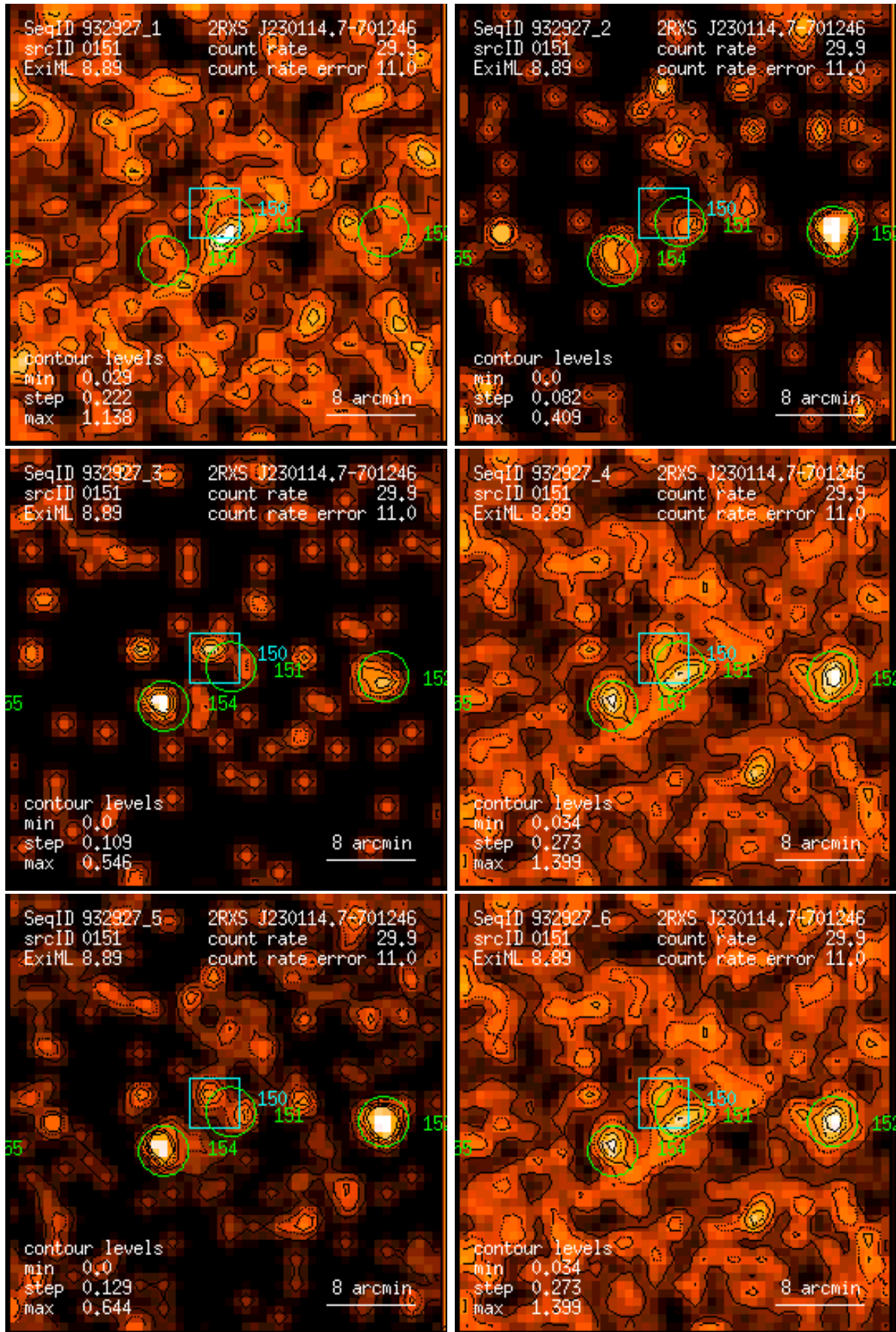
Figure 151: RASS 932927: detection 0151: band rate images, Gaussian filter: (1) PSPC channels 11 – 41, (2) 52 – 90, (3) 91 – 201, (4) 11 – 235, (5) 52 – 201, (6) 11 – 201. Broad band rates in counts/ks. Band rate contour levels in counts/ks/arcmin 2 .
