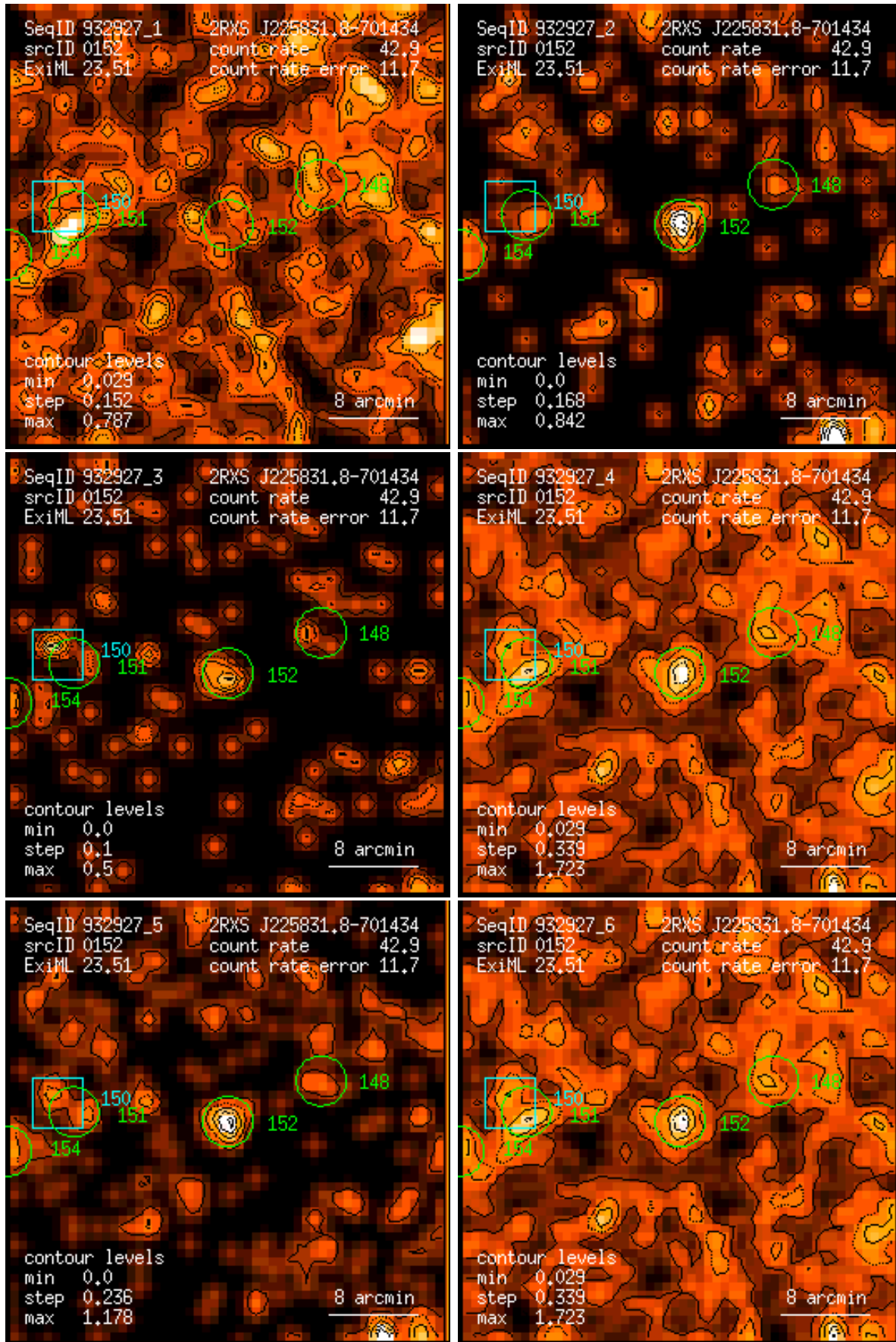
Figure 152: RASS 932927: detection 0152: band rate images, Gaussian filter: (1) PSPC channels 11 – 41, (2) 52 – 90, (3) 91 – 201, (4) 11 – 235, (5) 52 – 201, (6) 11 – 201. Broad band rates in counts/ks. Band rate contour levels in counts/ks/arcmin 2 .
