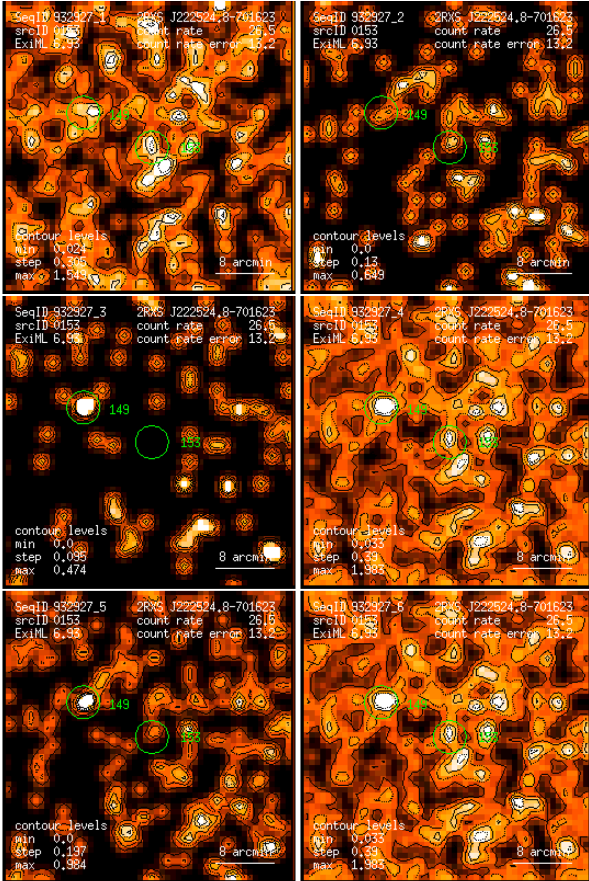
Figure 153: RASS 932927: detection 0153: band rate images, Gaussian filter: (1) PSPC channels 11 – 41, (2) 52 – 90, (3) 91 – 201, (4) 11 – 235, (5) 52 – 201, (6) 11 – 201. Broad band rates in counts/ks. Band rate contour levels in counts/ks/arcmin 2 .
