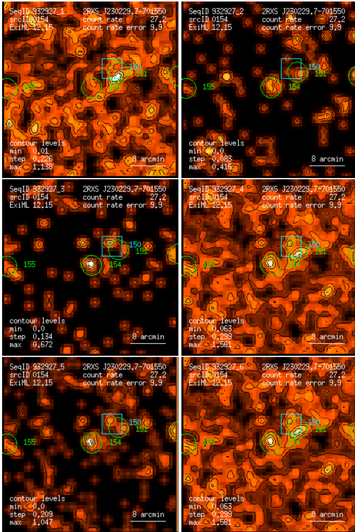
Figure 154: RASS 932927: detection 0154: band rate images, Gaussian filter: (1) PSPC channels 11 – 41, (2) 52 – 90, (3) 91 – 201, (4) 11 – 235, (5) 52 – 201, (6) 11 – 201. Broad band rates in counts/ks. Band rate contour levels in counts/ks/arcmin 2 .
