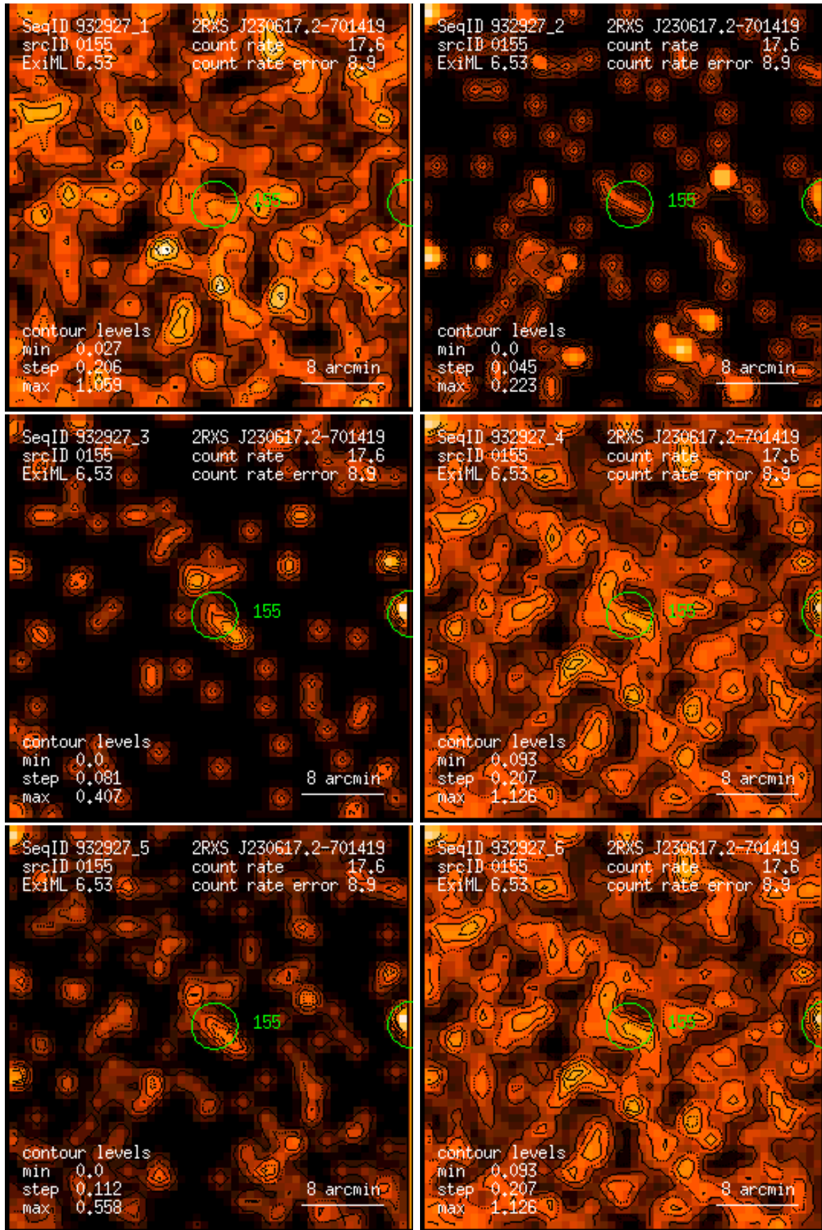
Figure 155: RASS 932927: detection 0155: band rate images, Gaussian filter: (1) PSPC channels 11 – 41, (2) 52 – 90, (3) 91 – 201, (4) 11 – 235, (5) 52 – 201, (6) 11 – 201. Broad band rates in counts/ks. Band rate contour levels in counts/ks/arcmin 2 .
