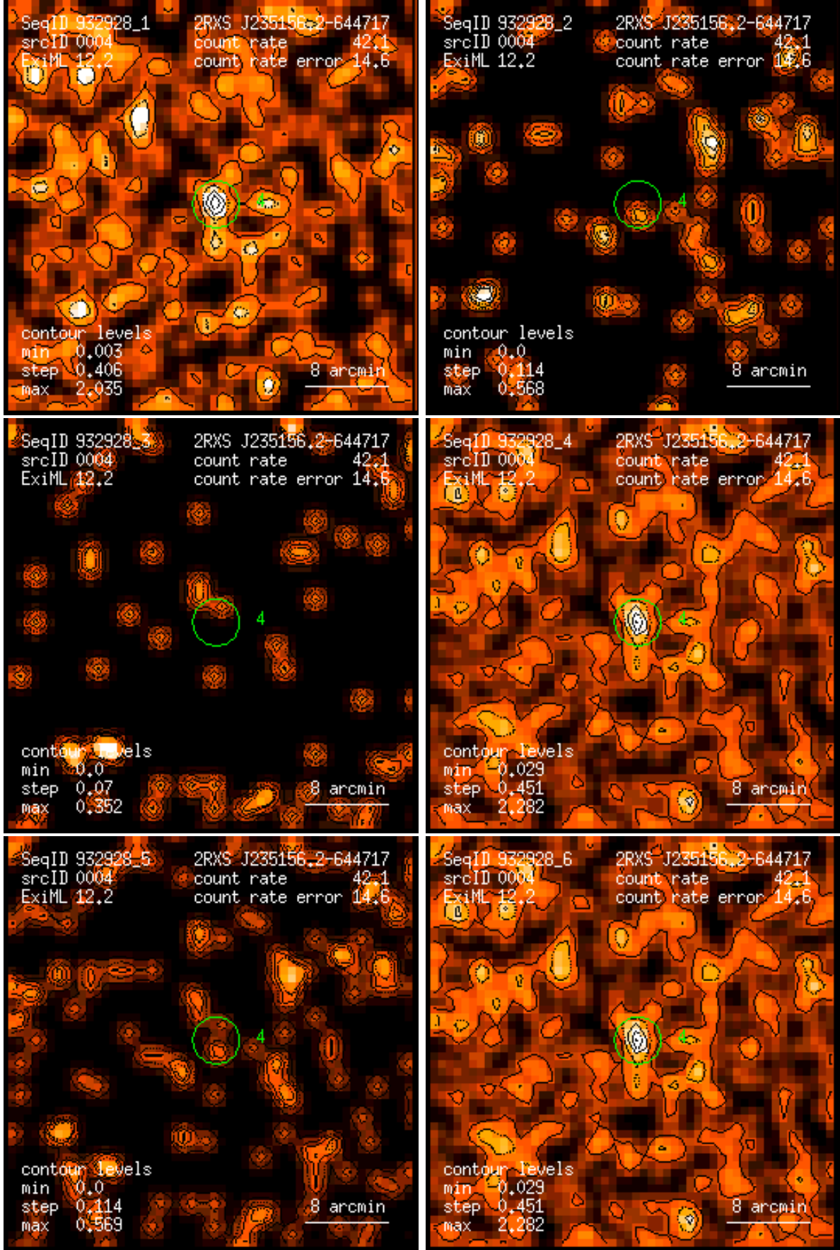
Figure 4: RASS 932928: detection 0004: band rate images, Gaussian filter: (1) PSPC channels 11 – 41, (2) 52 – 90, (3) 91 – 201, (4) 11 – 235, (5) 52 – 201, (6) 11 – 201. Broad band rates in counts/ks. Band rate contour levels in counts/ks/arcmin 2 .
