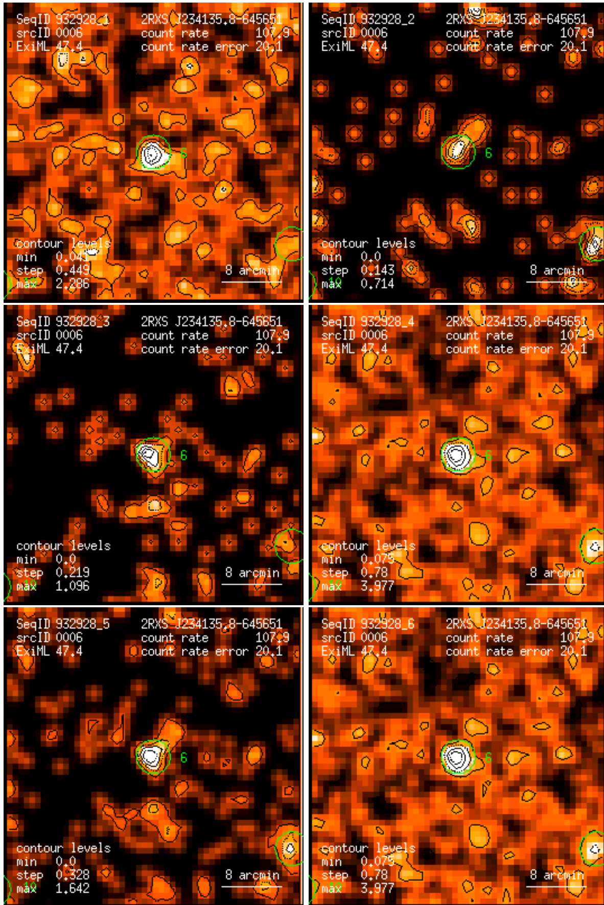
Figure 6: RASS 932928: detection 0006: band rate images, Gaussian filter: (1) PSPC channels 11 – 41, (2) 52 – 90, (3) 91 – 201, (4) 11 – 235, (5) 52 – 201, (6) 11 – 201. Broad band rates in counts/ks. Band rate contour levels in counts/ks/arcmin 2 .
