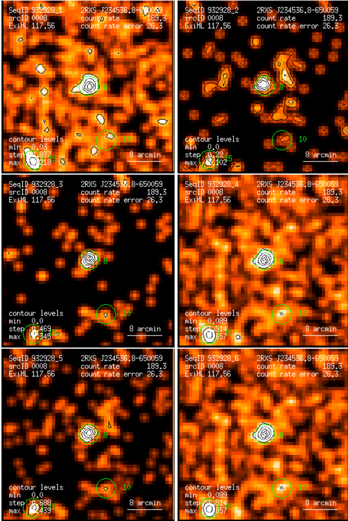
Figure 8: RASS 932928: detection 0008: band rate images, Gaussian filter: (1) PSPC channels 11 – 41, (2) 52 – 90, (3) 91 – 201, (4) 11 – 235, (5) 52 – 201, (6) 11 – 201. Broad band rates in counts/ks. Band rate contour levels in counts/ks/arcmin 2 .
