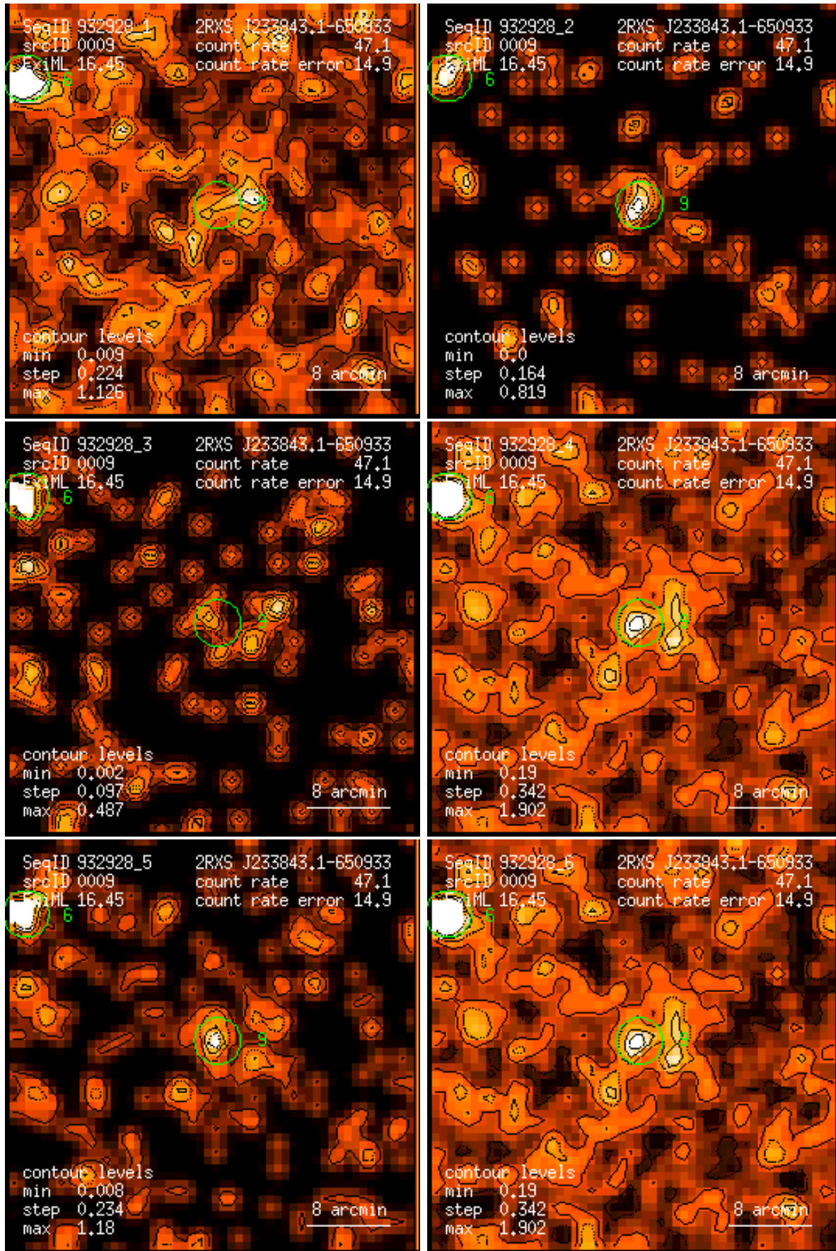
Figure 9: RASS 932928: detection 0009: band rate images, Gaussian filter: (1) PSPC channels 11 – 41, (2) 52 – 90, (3) 91 – 201, (4) 11 – 235, (5) 52 – 201, (6) 11 – 201. Broad band rates in counts/ks. Band rate contour levels in counts/ks/arcmin 2 .
