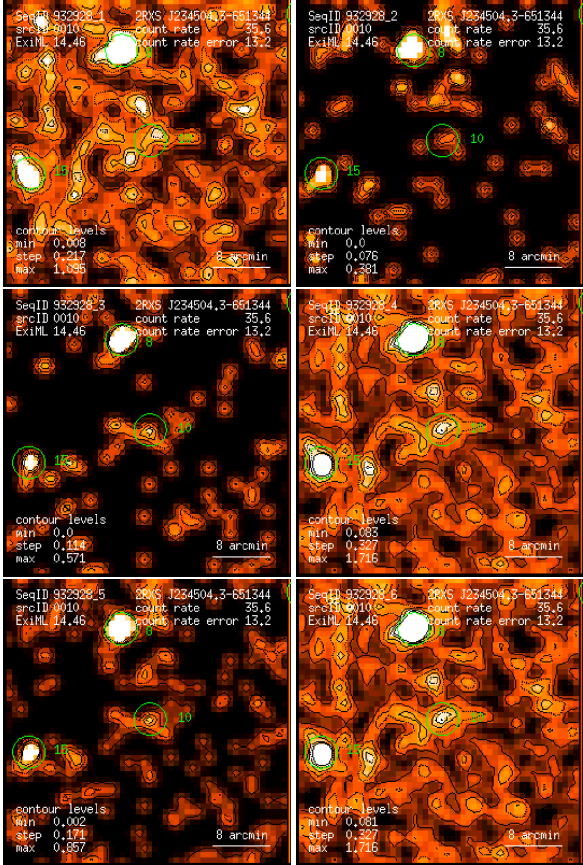
Figure 10: RASS 932928: detection 0010: band rate images, Gaussian filter: (1) PSPC channels 11 – 41, (2) 52 – 90, (3) 91 – 201, (4) 11 – 235, (5) 52 – 201, (6) 11 – 201. Broad band rates in counts/ks. Band rate contour levels in counts/ks/arcmin 2 .
