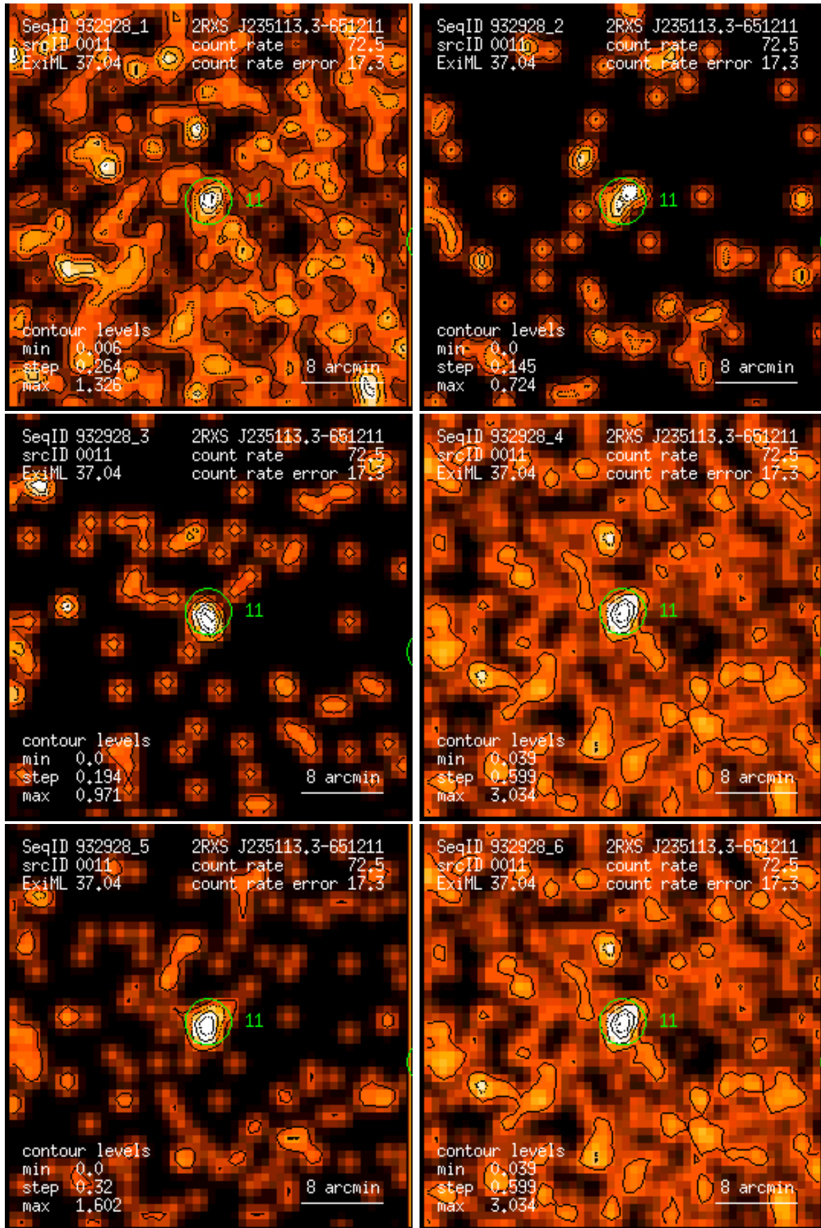
Figure 11: RASS 932928: detection 0011: band rate images, Gaussian filter: (1) PSPC channels 11 – 41, (2) 52 – 90, (3) 91 – 201, (4) 11 – 235, (5) 52 – 201, (6) 11 – 201. Broad band rates in counts/ks. Band rate contour levels in counts/ks/arcmin 2 .
