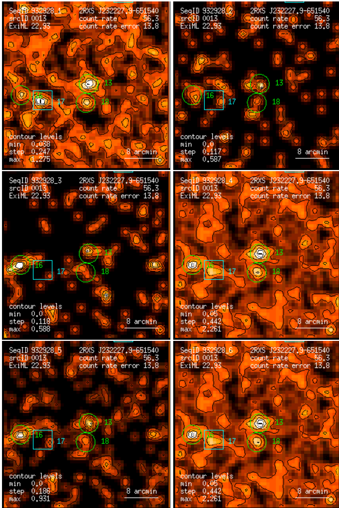
Figure 13: RASS 932928: detection 0013: band rate images, Gaussian filter: (1) PSPC channels 11 – 41, (2) 52 – 90, (3) 91 – 201, (4) 11 – 235, (5) 52 – 201, (6) 11 – 201. Broad band rates in counts/ks. Band rate contour levels in counts/ks/arcmin 2 .
