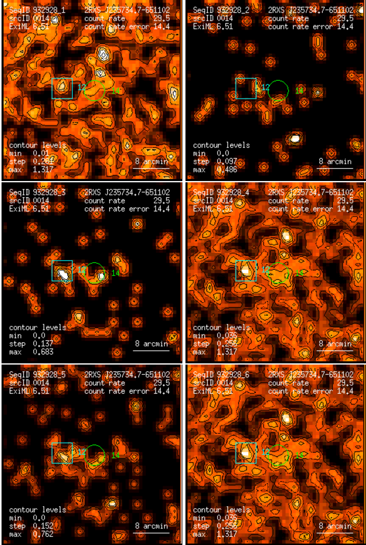
Figure 14: RASS 932928: detection 0014: band rate images, Gaussian filter: (1) PSPC channels 11 – 41, (2) 52 – 90, (3) 91 – 201, (4) 11 – 235, (5) 52 – 201, (6) 11 – 201. Broad band rates in counts/ks. Band rate contour levels in counts/ks/arcmin 2 .
