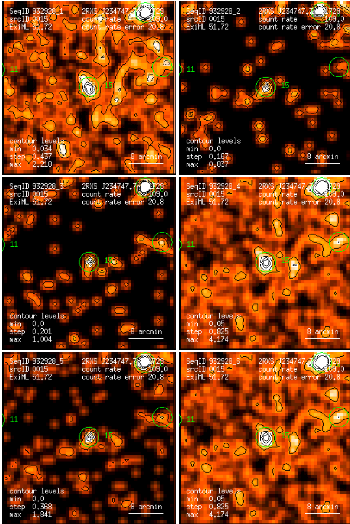
Figure 15: RASS 932928: detection 0015: band rate images, Gaussian filter: (1) PSPC channels 11 – 41, (2) 52 – 90, (3) 91 – 201, (4) 11 – 235, (5) 52 – 201, (6) 11 – 201. Broad band rates in counts/ks. Band rate contour levels in counts/ks/arcmin 2 .
