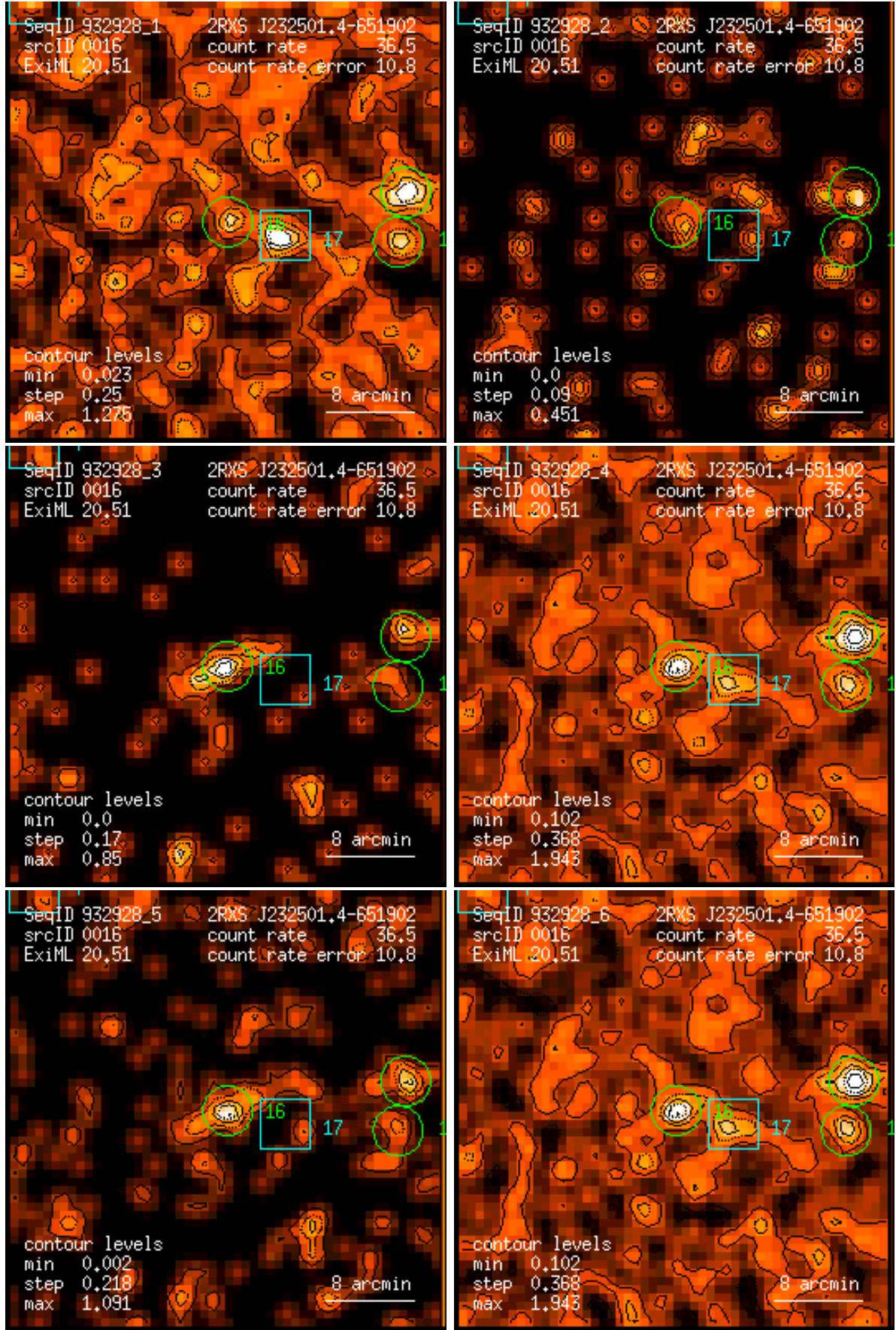
Figure 16: RASS 932928: detection 0016: band rate images, Gaussian filter: (1) PSPC channels 11 – 41, (2) 52 – 90, (3) 91 – 201, (4) 11 – 235, (5) 52 – 201, (6) 11 – 201. Broad band rates in counts/ks. Band rate contour levels in counts/ks/arcmin 2 .
