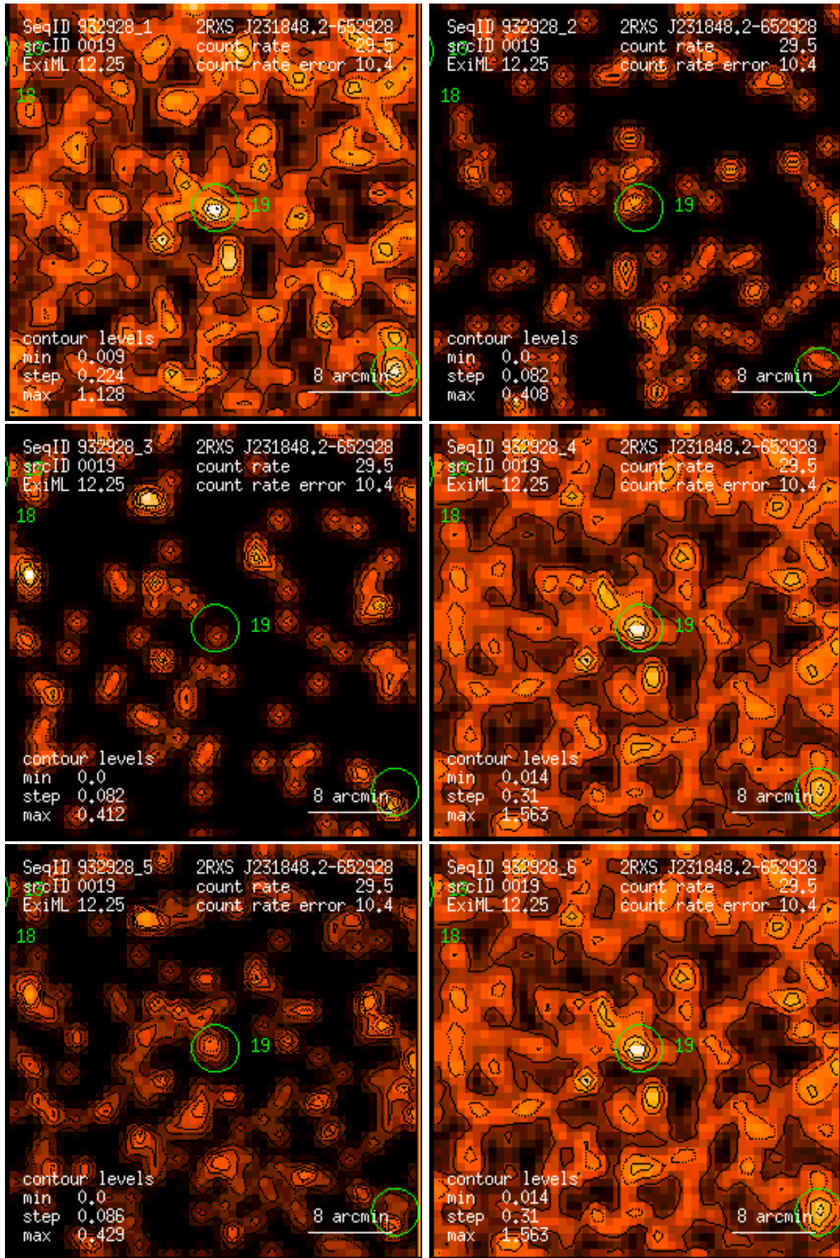
Figure 19: RASS 932928: detection 0019: band rate images, Gaussian filter: (1) PSPC channels 11 – 41, (2) 52 – 90, (3) 91 – 201, (4) 11 – 235, (5) 52 – 201, (6) 11 – 201. Broad band rates in counts/ks. Band rate contour levels in counts/ks/arcmin 2 .
