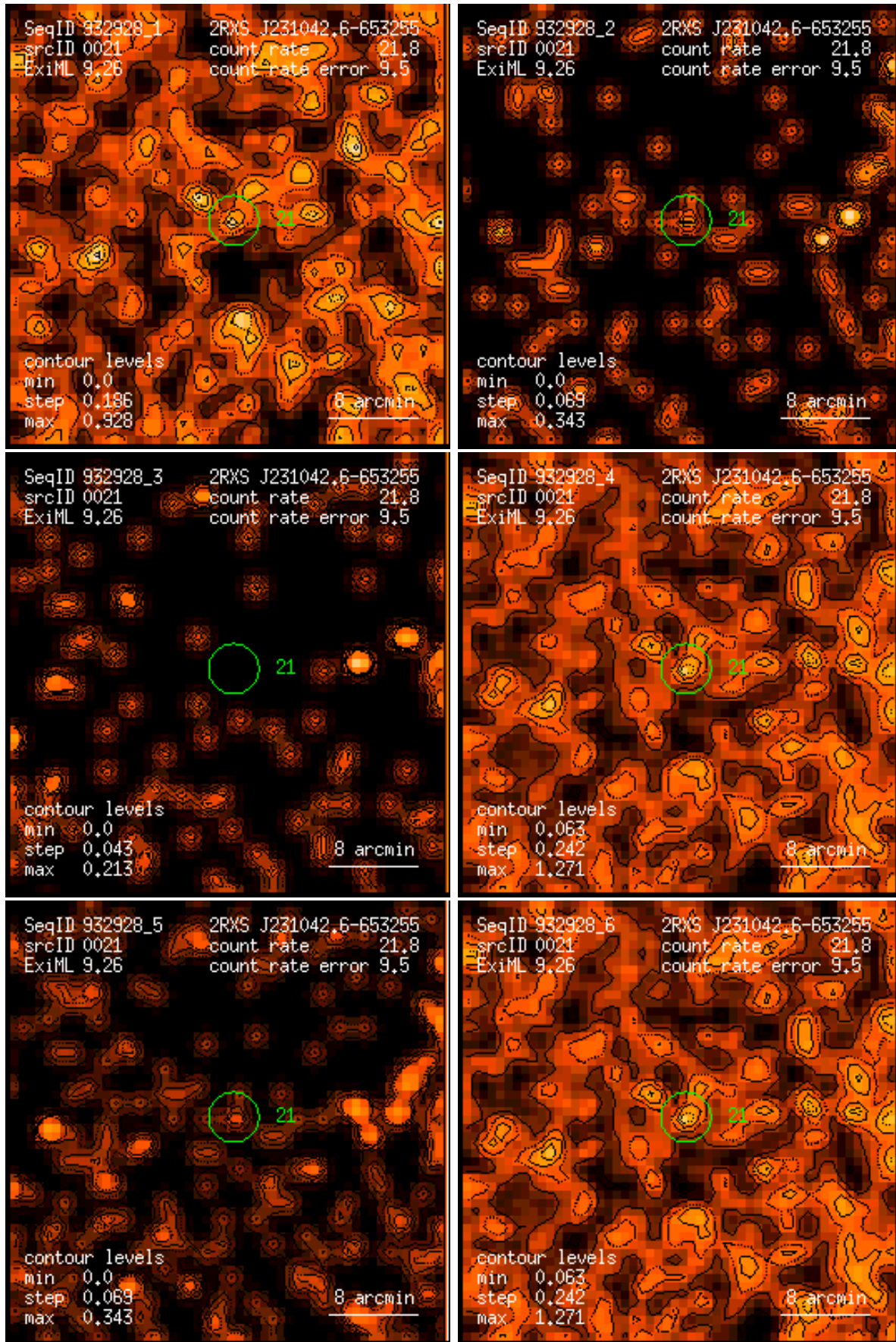
Figure 21: RASS 932928: detection 0021: band rate images, Gaussian filter: (1) PSPC channels 11 – 41, (2) 52 – 90, (3) 91 – 201, (4) 11 – 235, (5) 52 – 201, (6) 11 – 201. Broad band rates in counts/ks. Band rate contour levels in counts/ks/arcmin 2 .
