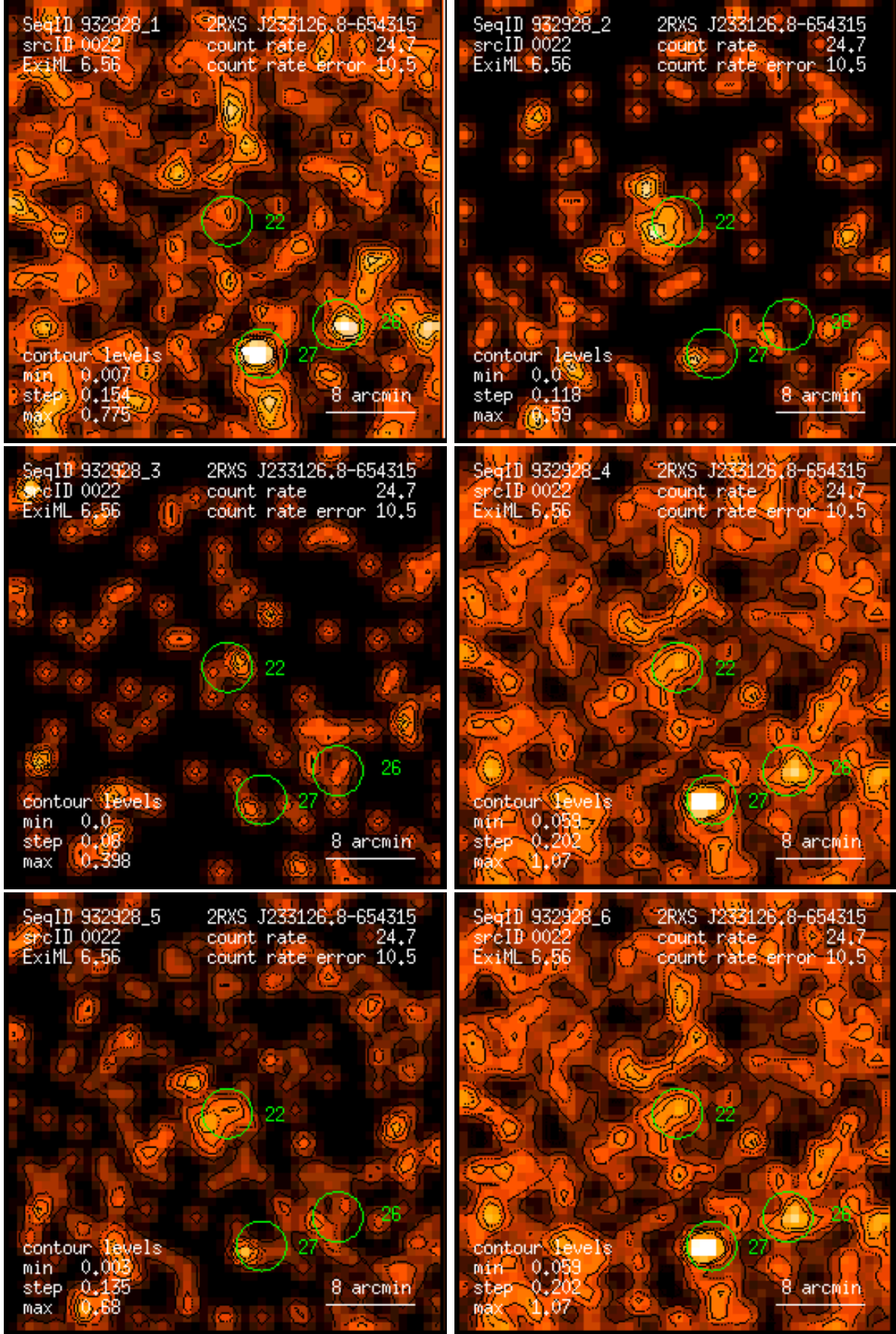
Figure 22: RASS 932928: detection 0022: band rate images, Gaussian filter: (1) PSPC channels 11 – 41, (2) 52 – 90, (3) 91 – 201, (4) 11 – 235, (5) 52 – 201, (6) 11 – 201. Broad band rates in counts/ks. Band rate contour levels in counts/ks/arcmin 2 .
