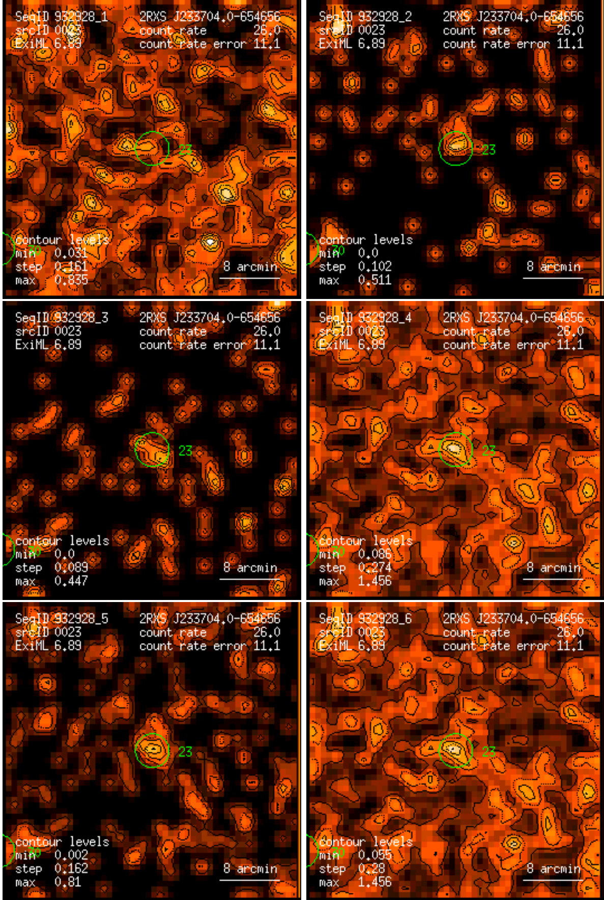
Figure 23: RASS 932928: detection 0023: band rate images, Gaussian filter: (1) PSPC channels 11 – 41, (2) 52 – 90, (3) 91 – 201, (4) 11 – 235, (5) 52 – 201, (6) 11 – 201. Broad band rates in counts/ks. Band rate contour levels in counts/ks/arcmin 2 .
