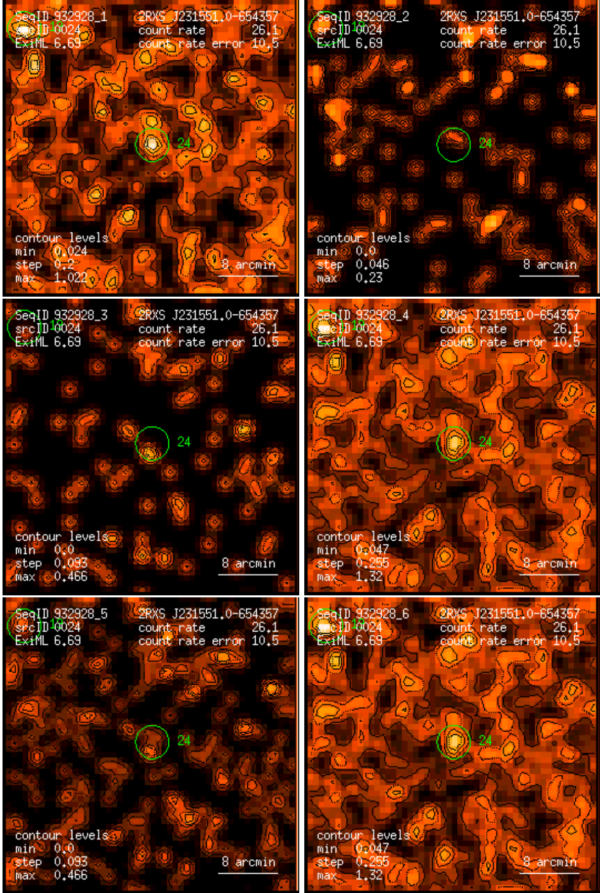
Figure 24: RASS 932928: detection 0024: band rate images, Gaussian filter: (1) PSPC channels 11 – 41, (2) 52 – 90, (3) 91 – 201, (4) 11 – 235, (5) 52 – 201, (6) 11 – 201. Broad band rates in counts/ks. Band rate contour levels in counts/ks/arcmin 2 .
