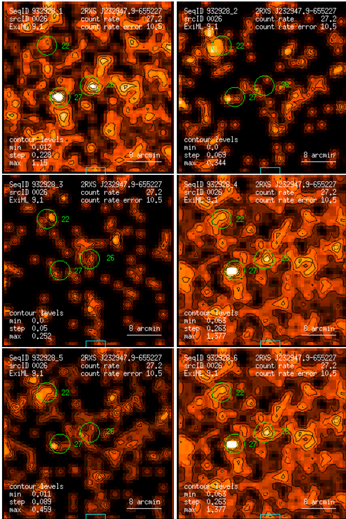
Figure 26: RASS 932928: detection 0026: band rate images, Gaussian filter: (1) PSPC channels 11 – 41, (2) 52 – 90, (3) 91 – 201, (4) 11 – 235, (5) 52 – 201, (6) 11 – 201. Broad band rates in counts/ks. Band rate contour levels in counts/ks/arcmin 2 .
