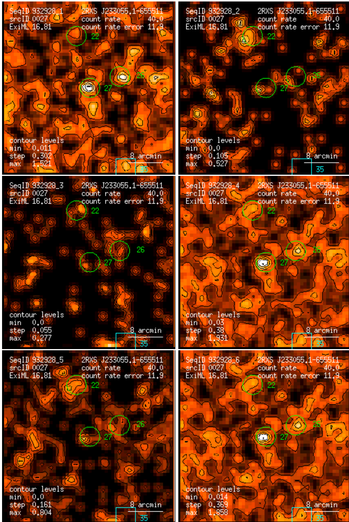
Figure 27: RASS 932928: detection 0027: band rate images, Gaussian filter: (1) PSPC channels 11 – 41, (2) 52 – 90, (3) 91 – 201, (4) 11 – 235, (5) 52 – 201, (6) 11 – 201. Broad band rates in counts/ks. Band rate contour levels in counts/ks/arcmin 2 .
