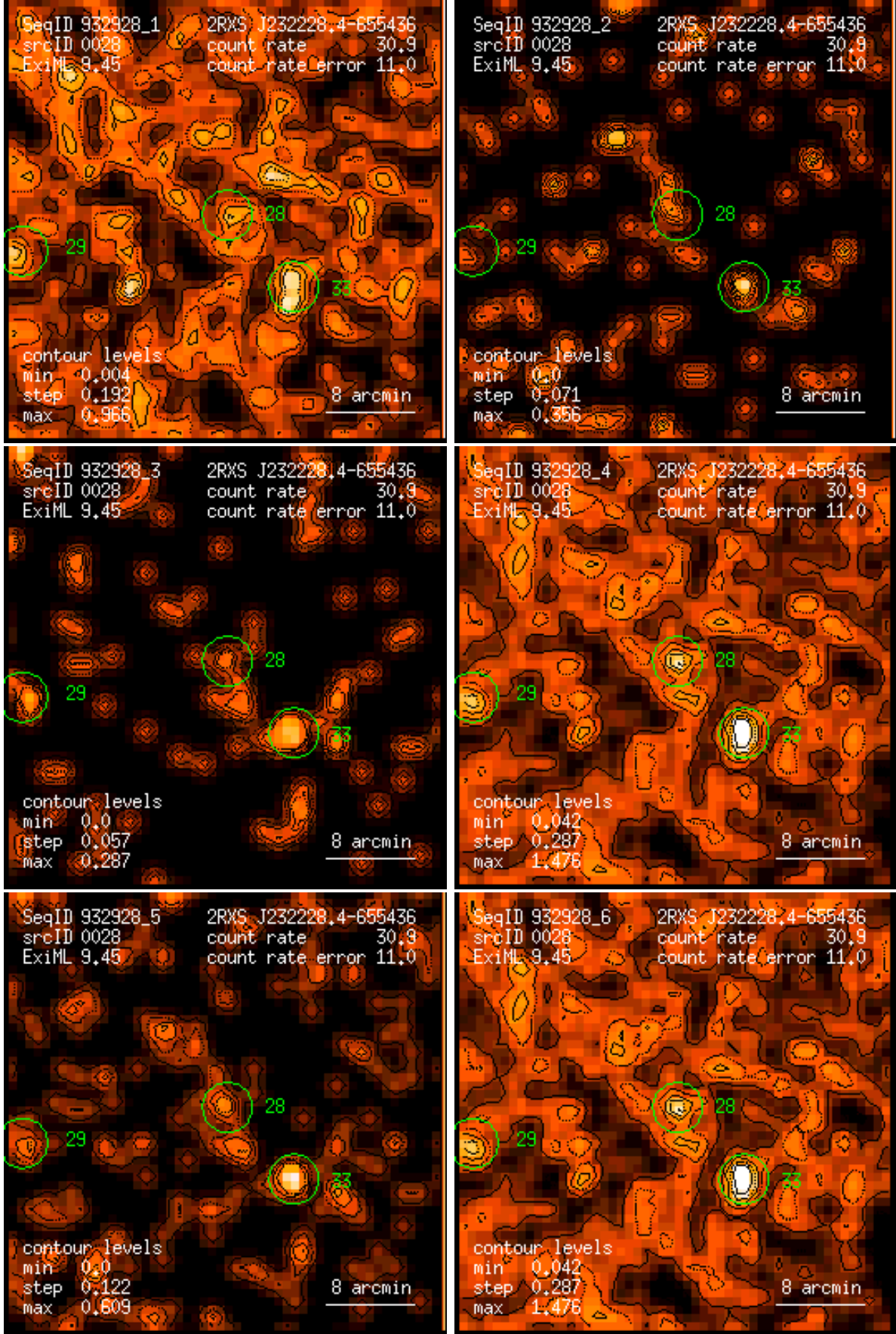
Figure 28: RASS 932928: detection 0028: band rate images, Gaussian filter: (1) PSPC channels 11 – 41, (2) 52 – 90, (3) 91 – 201, (4) 11 – 235, (5) 52 – 201, (6) 11 – 201. Broad band rates in counts/ks. Band rate contour levels in counts/ks/arcmin 2 .
