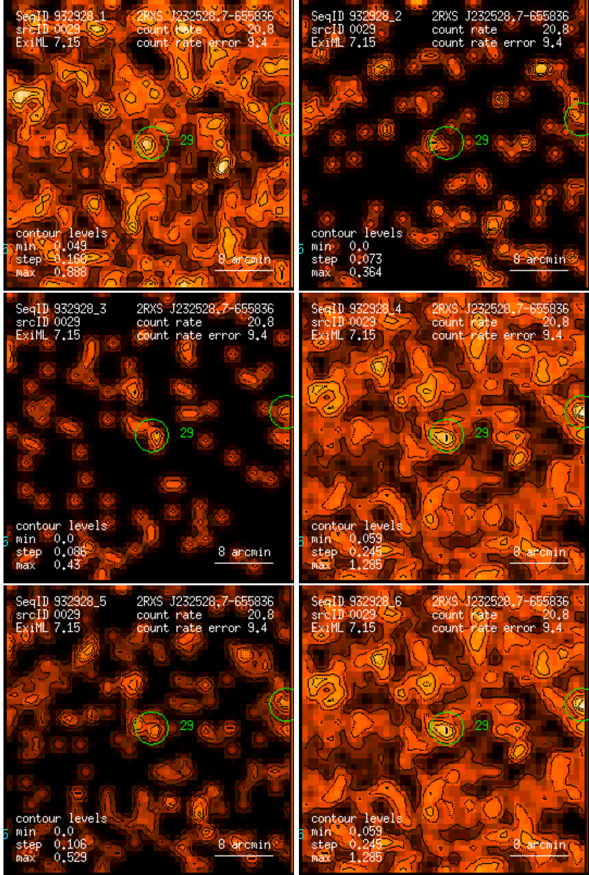
Figure 29: RASS 932928: detection 0029: band rate images, Gaussian filter: (1) PSPC channels 11 – 41, (2) 52 – 90, (3) 91 – 201, (4) 11 – 235, (5) 52 – 201, (6) 11 – 201. Broad band rates in counts/ks. Band rate contour levels in counts/ks/arcmin 2 .
