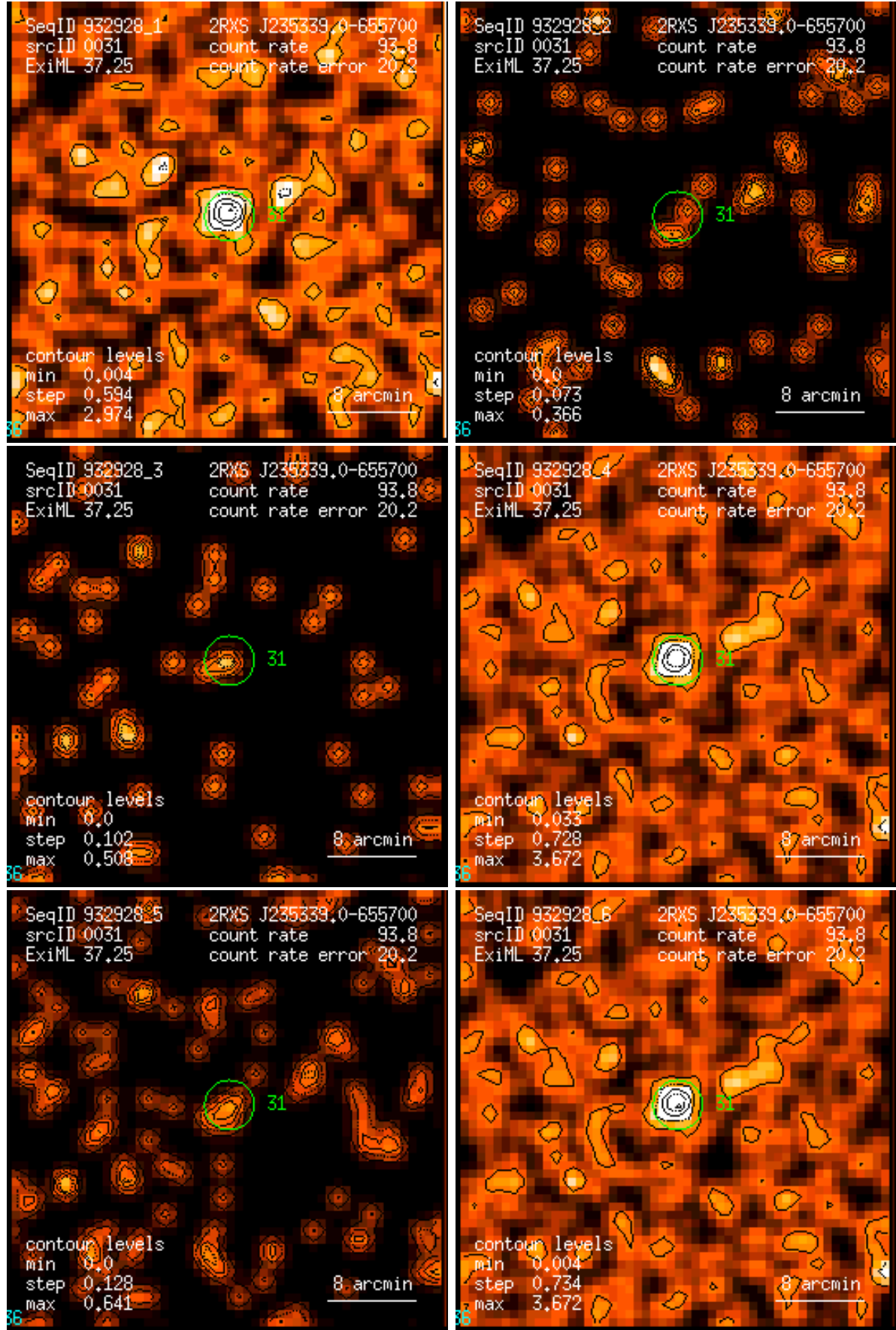
Figure 31: RASS 932928: detection 0031: band rate images, Gaussian filter: (1) PSPC channels 11 – 41, (2) 52 – 90, (3) 91 – 201, (4) 11 – 235, (5) 52 – 201, (6) 11 – 201. Broad band rates in counts/ks. Band rate contour levels in counts/ks/arcmin 2 .
