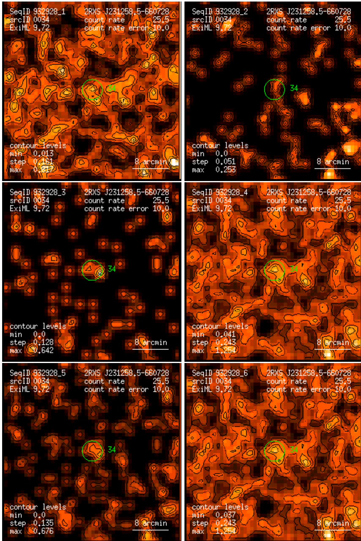
Figure 34: RASS 932928: detection 0034: band rate images, Gaussian filter: (1) PSPC channels 11 – 41, (2) 52 – 90, (3) 91 – 201, (4) 11 – 235, (5) 52 – 201, (6) 11 – 201. Broad band rates in counts/ks. Band rate contour levels in counts/ks/arcmin 2 .
