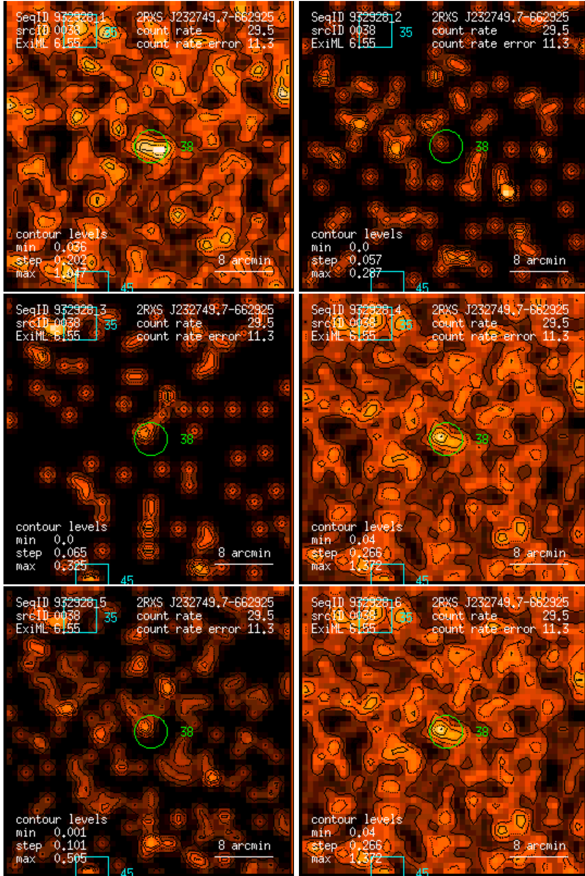
Figure 38: RASS 932928: detection 0038: band rate images, Gaussian filter: (1) PSPC channels 11 – 41, (2) 52 – 90, (3) 91 – 201, (4) 11 – 235, (5) 52 – 201, (6) 11 – 201. Broad band rates in counts/ks. Band rate contour levels in counts/ks/arcmin 2 .
