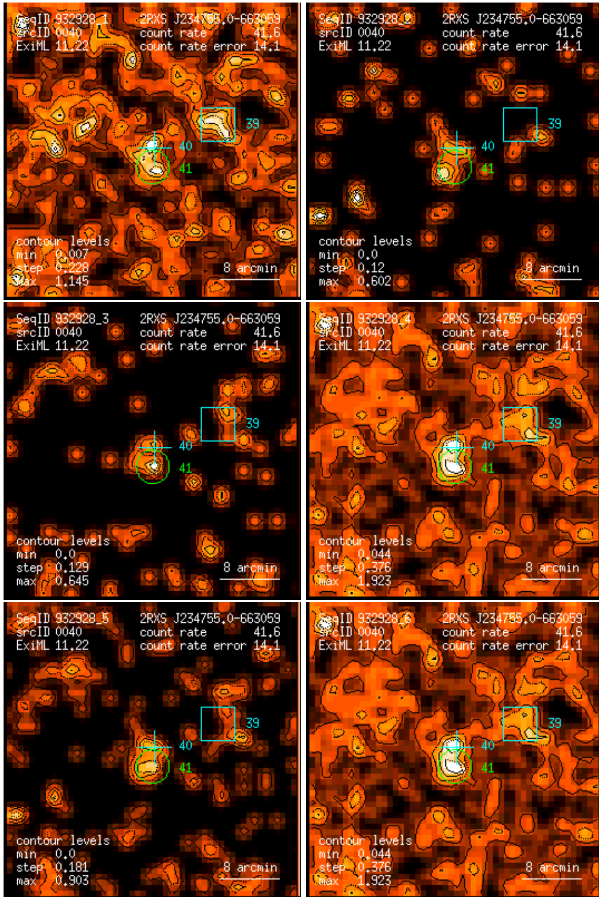
Figure 40: RASS 932928: detection 0040: band rate images, Gaussian filter: (1) PSPC channels 11 – 41, (2) 52 – 90, (3) 91 – 201, (4) 11 – 235, (5) 52 – 201, (6) 11 – 201. Broad band rates in counts/ks. Band rate contour levels in counts/ks/arcmin 2 .
