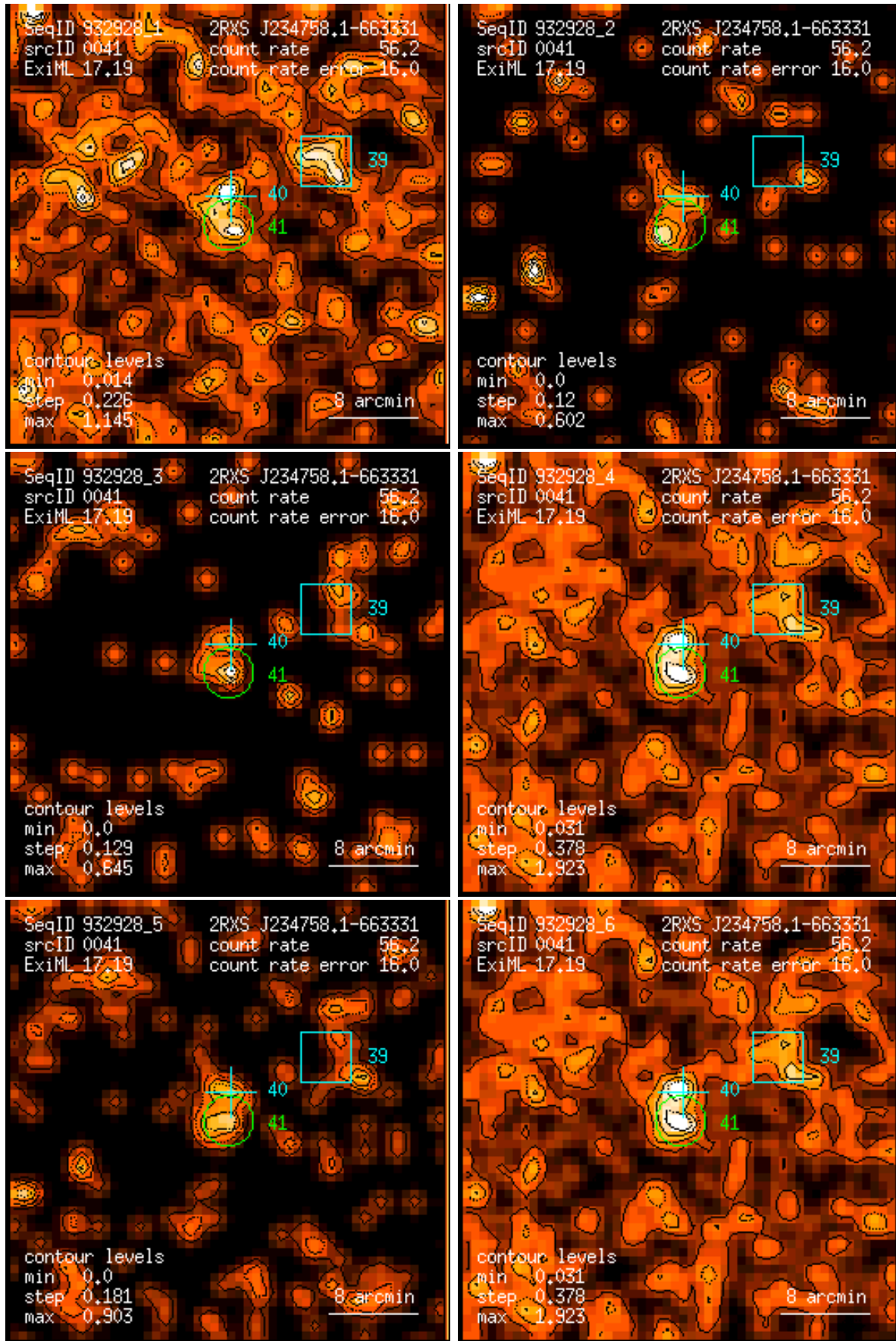
Figure 41: RASS 932928: detection 0041: band rate images, Gaussian filter: (1) PSPP channels 11 – 41, (2) 52 – 90, (3) 91 – 201, (4) 11 – 235, (5) 52 – 201, (6) 11 – 201. Broad band rates in counts/ks. Band rate contour levels in counts/ks/arcmin 2 .
