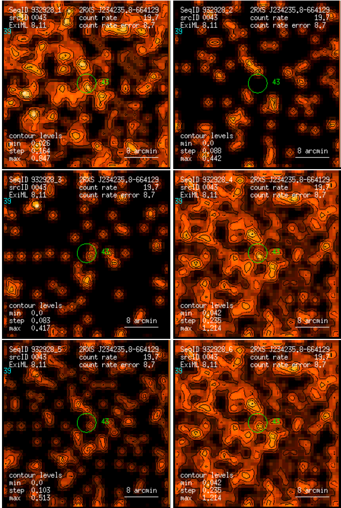
Figure 43: RASS 932928: detection 0043: band rate images, Gaussian filter: (1) PSPC channels 11 – 41, (2) 52 – 90, (3) 91 – 201, (4) 11 – 235, (5) 52 – 201, (6) 11 – 201. Broad band rates in counts/ks. Band rate contour levels in counts/ks/arcmin 2 .
