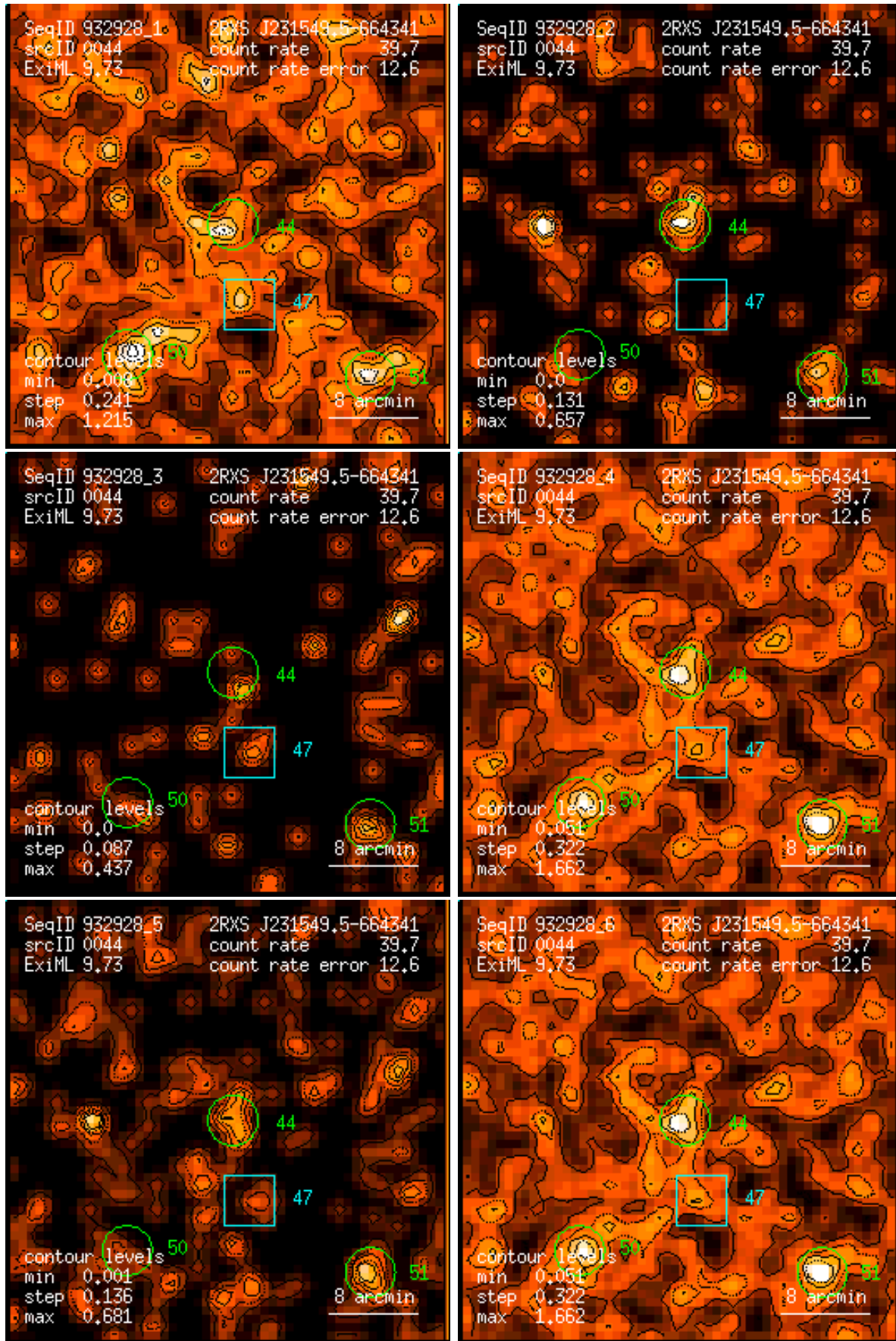
Figure 44: RASS 932928: detection 0044: band rate images, Gaussian filter: (1) PSPC channels 11 – 41, (2) 52 – 90, (3) 91 – 201, (4) 11 – 235, (5) 52 – 201, (6) 11 – 201. Broad band rates in counts/ks. Band rate contour levels in counts/ks/arcmin 2 .
